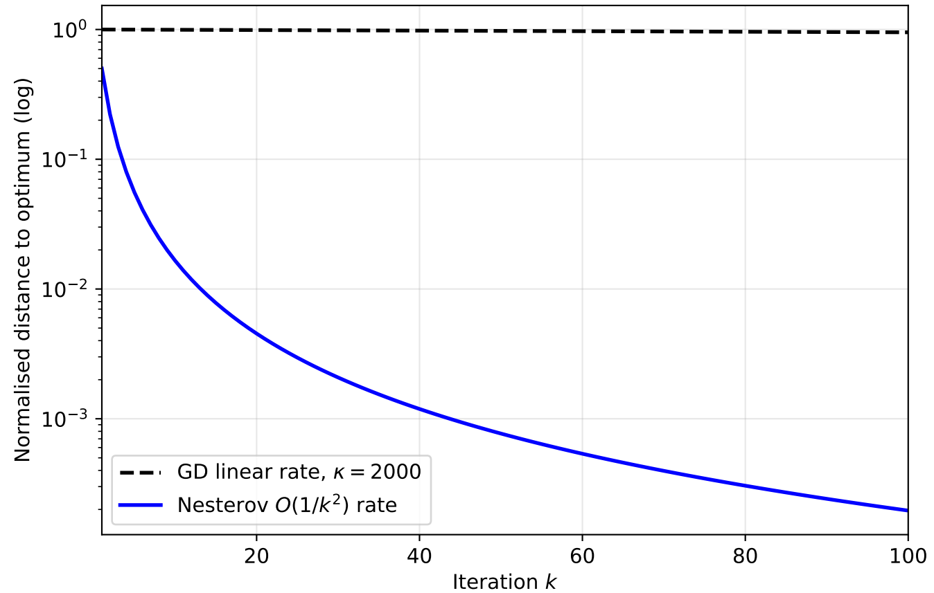
GD vs Nesterov Rate ( \kappa = 2000 )
