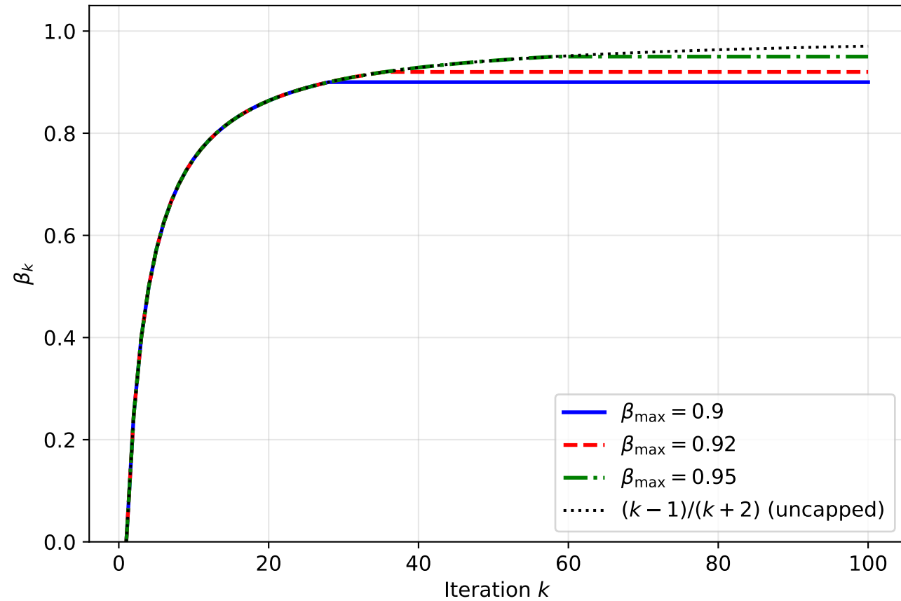
Nesterov Momentum Schedule \beta_k = \min((k-1)/(k+2), \beta_{\max})
