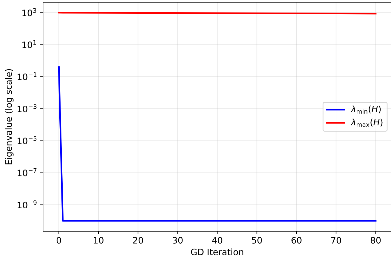
Rosenbrock: Hessian Eigenvalues Along GD Path
