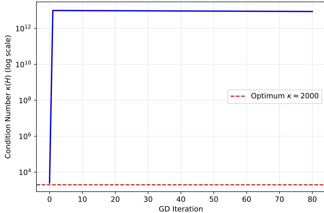
Rosenbrock: Hessian Condition Number Along GD Path
