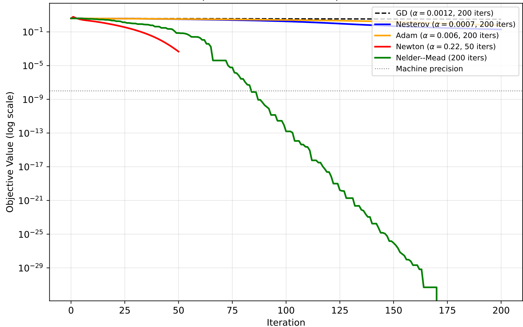
Rosenbrock: Comprehensive Method Comparison (200 Iterations)
