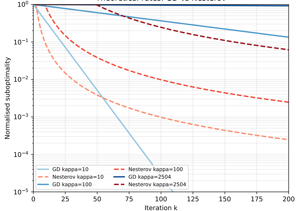
Theoretical rates: GD vs Nesterov
