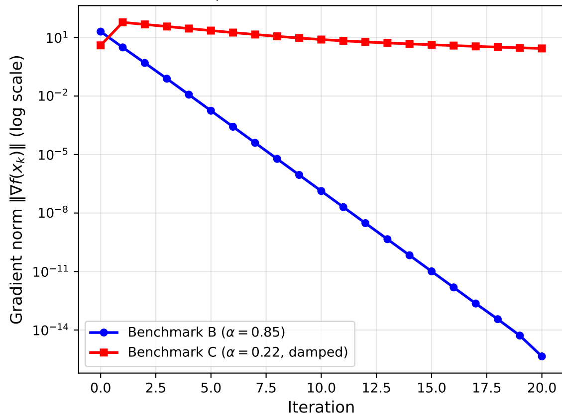
Q3: Newton's Method Gradient Norm Convex-quadratic vs Non-convex (Rosenbrock)
