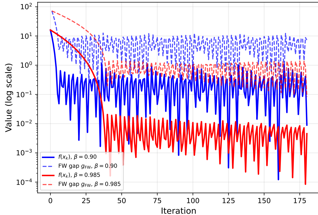
Q6-II: Frank-Wolfe Duality Gap Interior Optimum f(x) = (x_1 - 1)^2 + (x_2 - 5)^2
