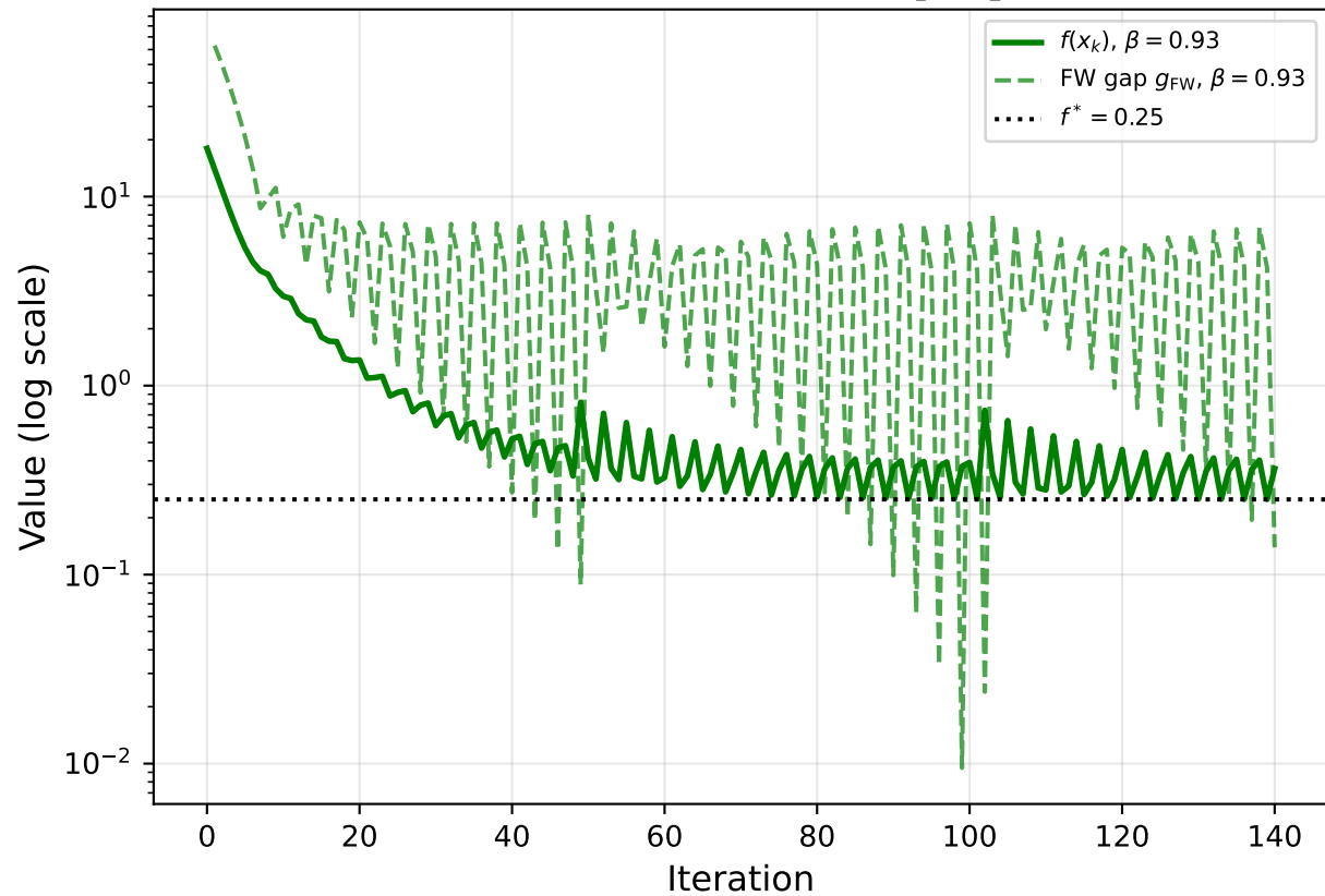
Q6-III: Frank-Wolfe Duality Gap Boundary Optimum f(x) = x_1^2 + x_2^2
