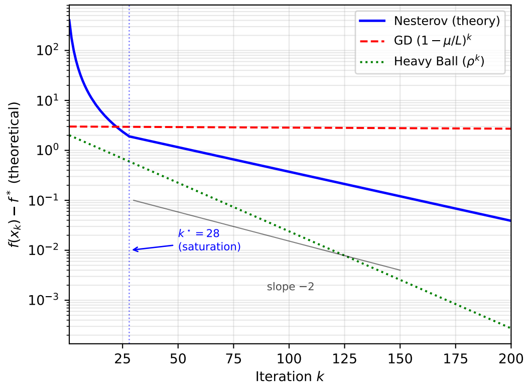
Two-phase Nesterov convergence ( \kappa = 2000 )
