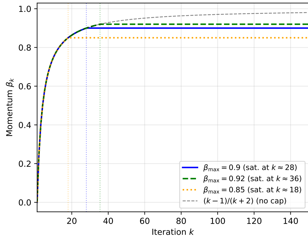
Nesterov \beta_k schedule with cap
