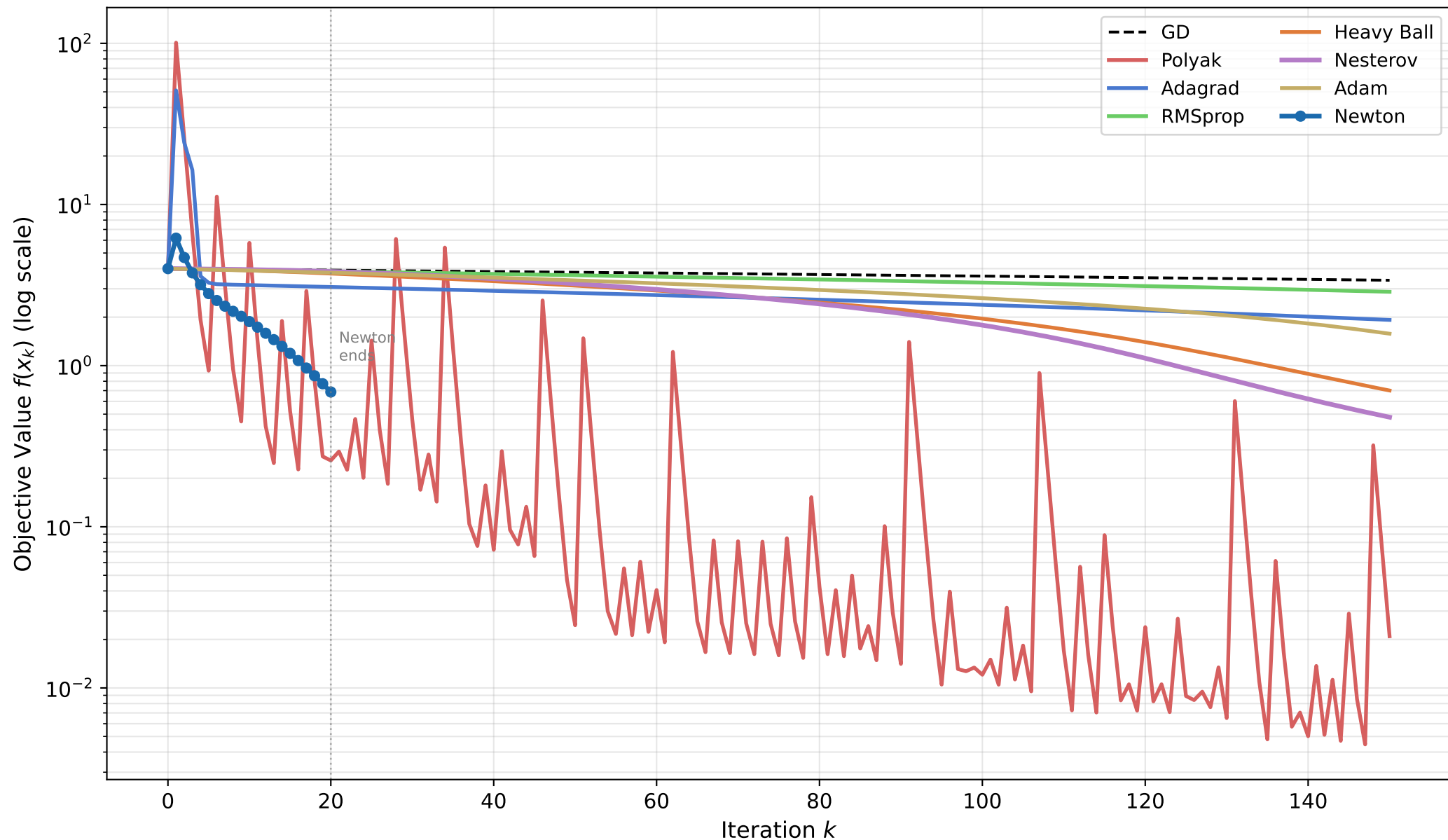
Benchmark C (Rosenbrock): All Methods Convergence Comparison First-order: 150 iterations; Newton: 20 iterations
