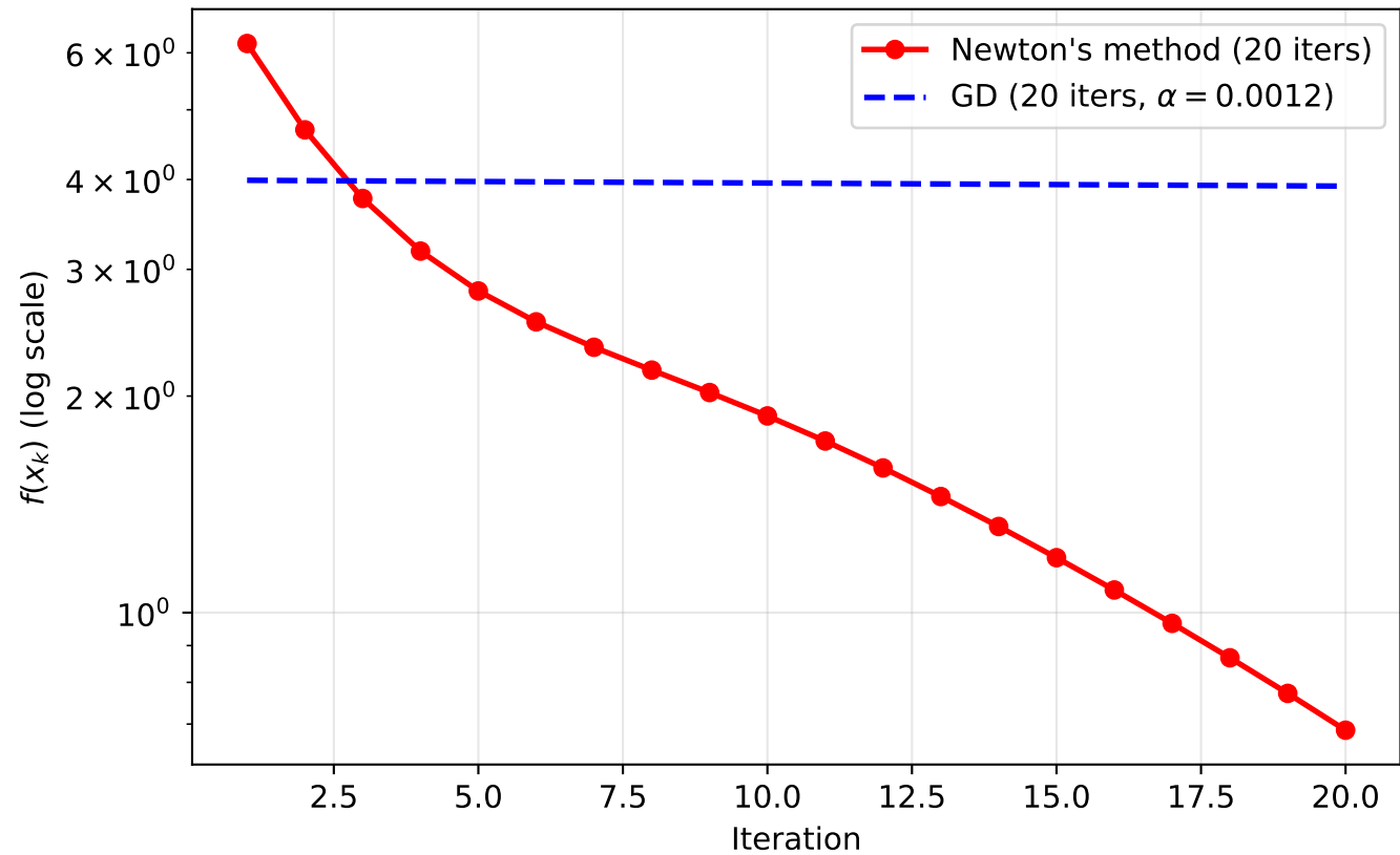
Newton vs GD: First 20 Iterations on Rosenbrock
