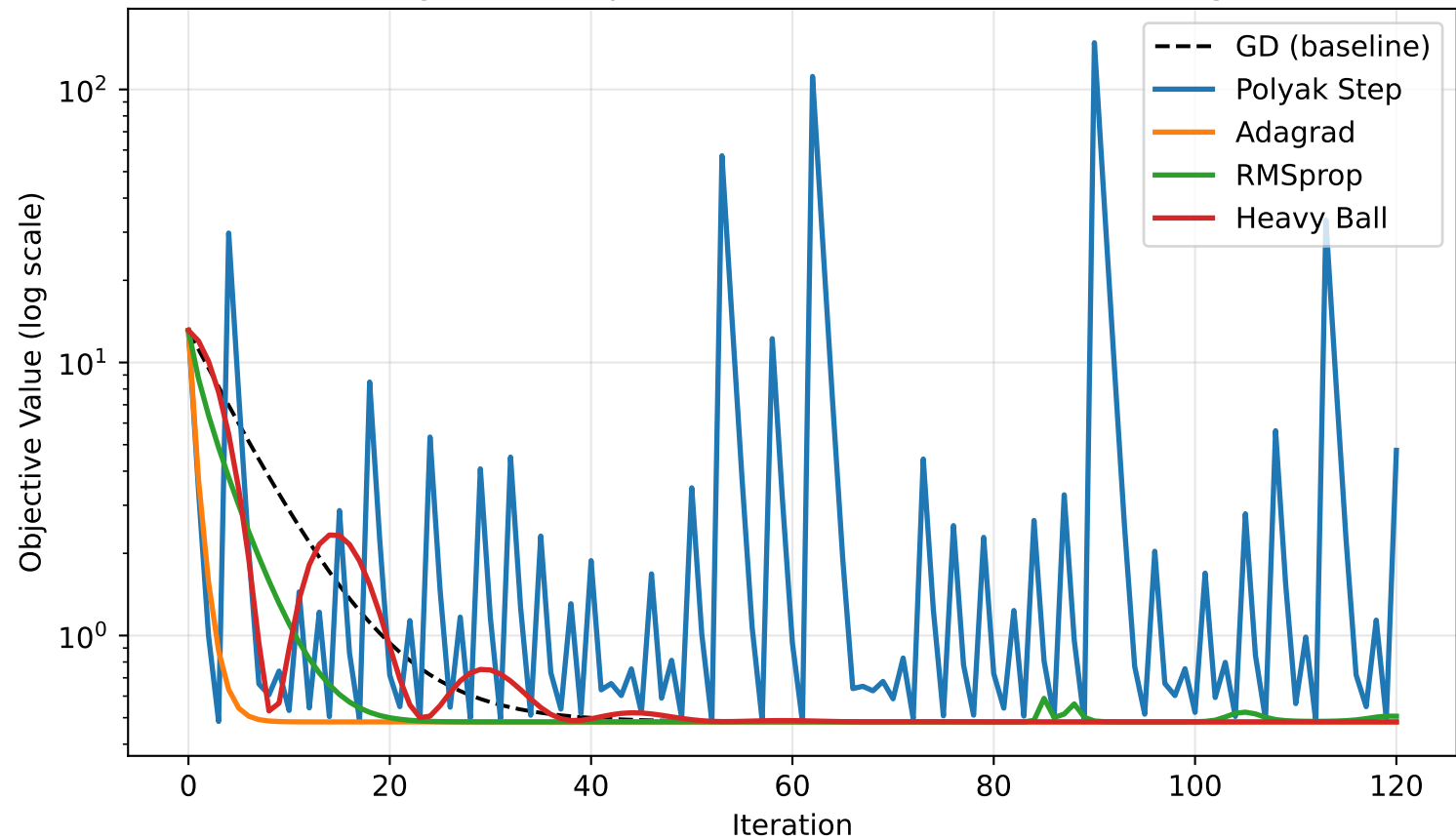
Q1: Convergence Comparison — Benchmark A (Linear Regression)
