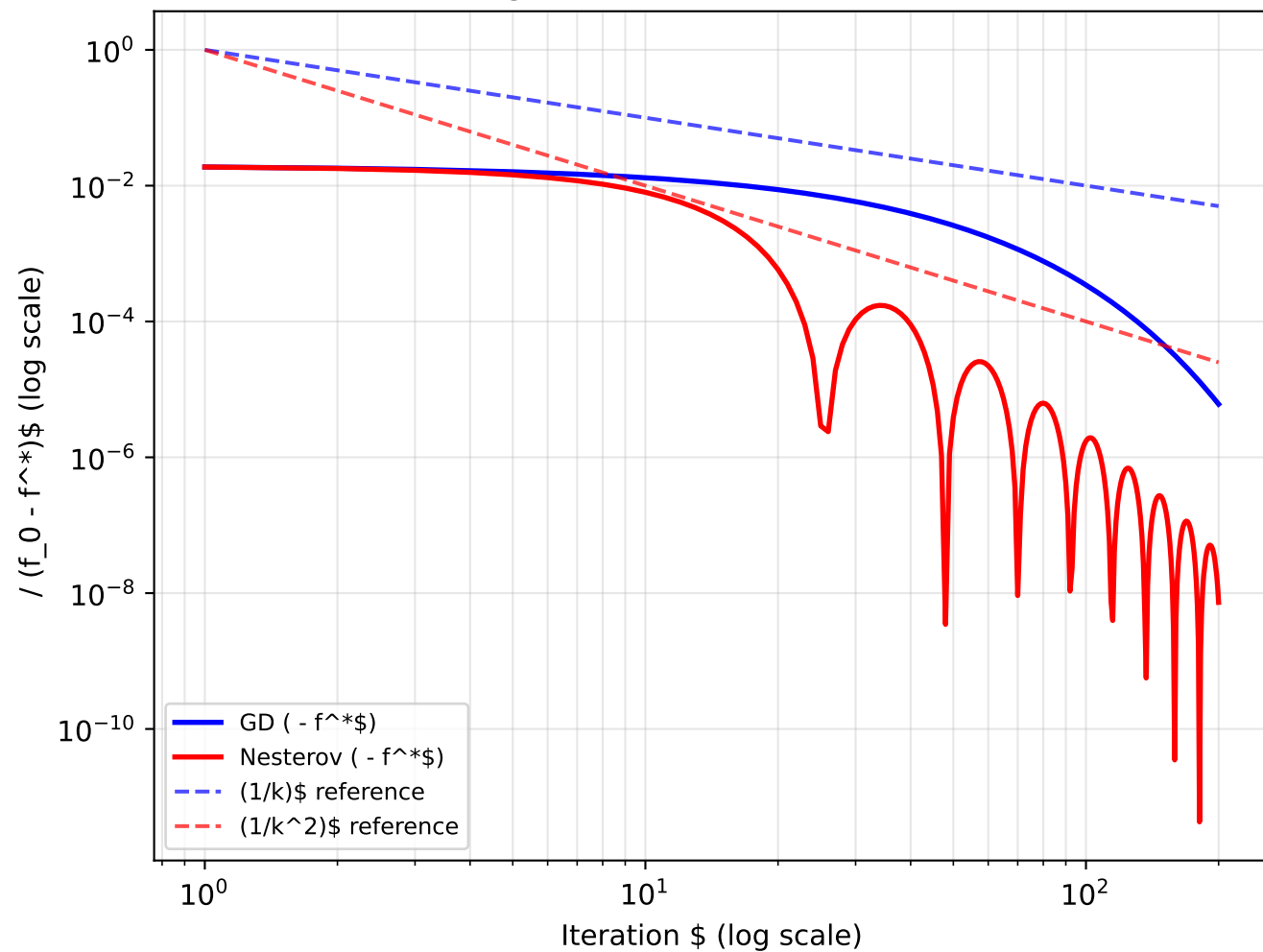
Convergence Rate Verification ( \kappa = 50 )
