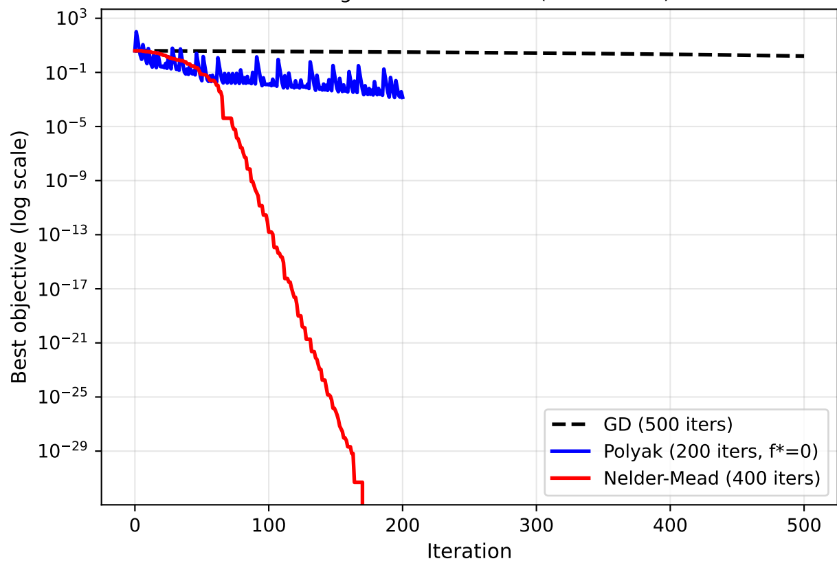
Convergence vs Iterations (Rosenbrock)
