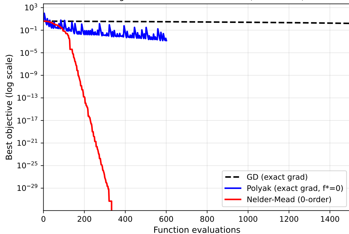
Convergence vs Function Evaluations (Rosenbrock)
