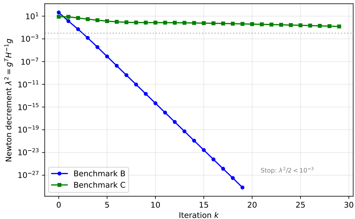
Newton Decrement vs. Iteration
