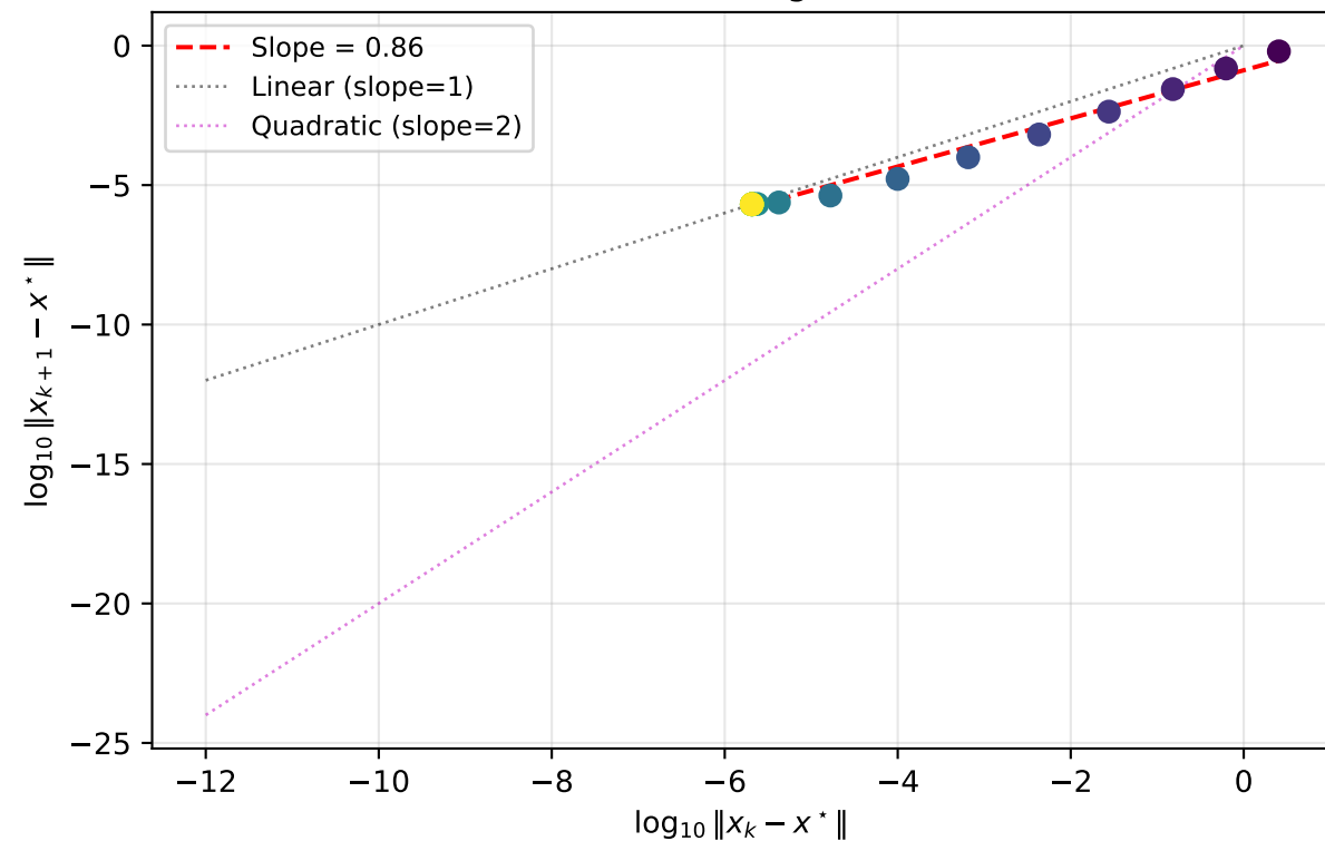
Newton: Quadratic Convergence Verification (B)
