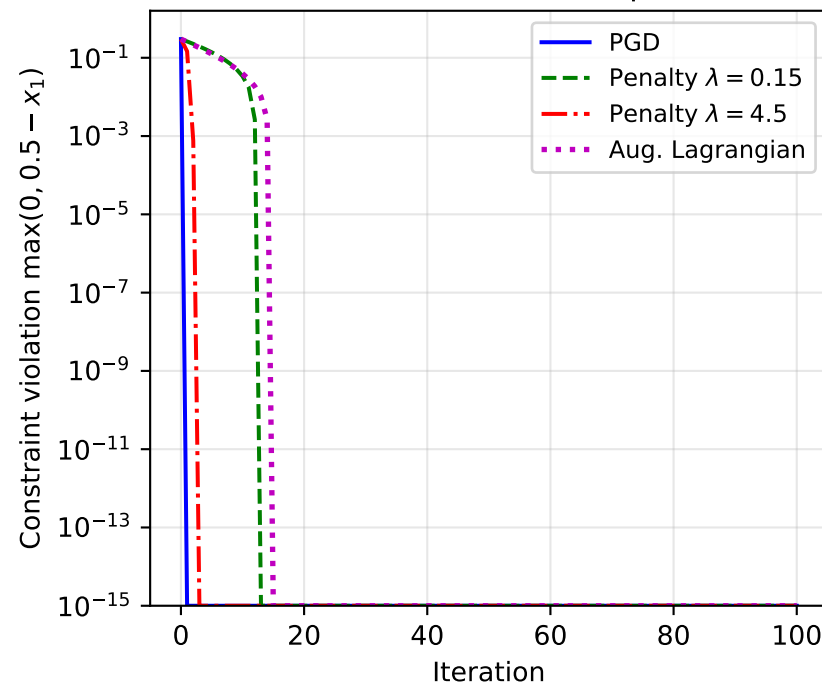
Constraint Violation Comparison
