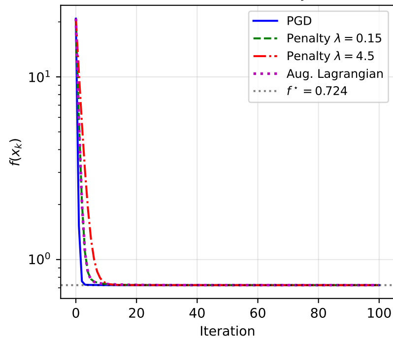
Constrained Methods: Objective
