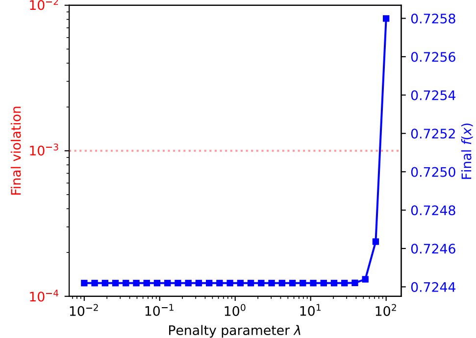
Penalty Method: \lambda Sensitivity (200 iters)
