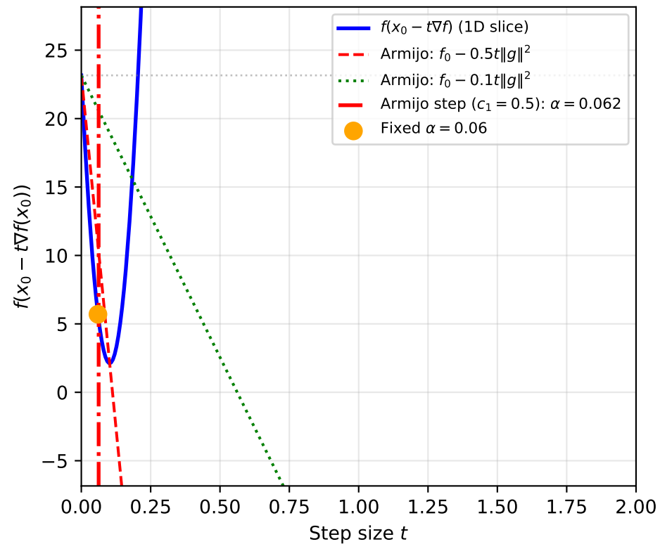
Armijo Sufficient Decrease Condition (1D slice at x_0 = [-1, 4]^T )
