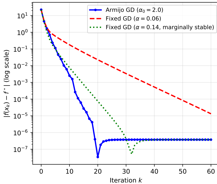
Armijo vs Fixed Step Size: Convergence (Benchmark B)
