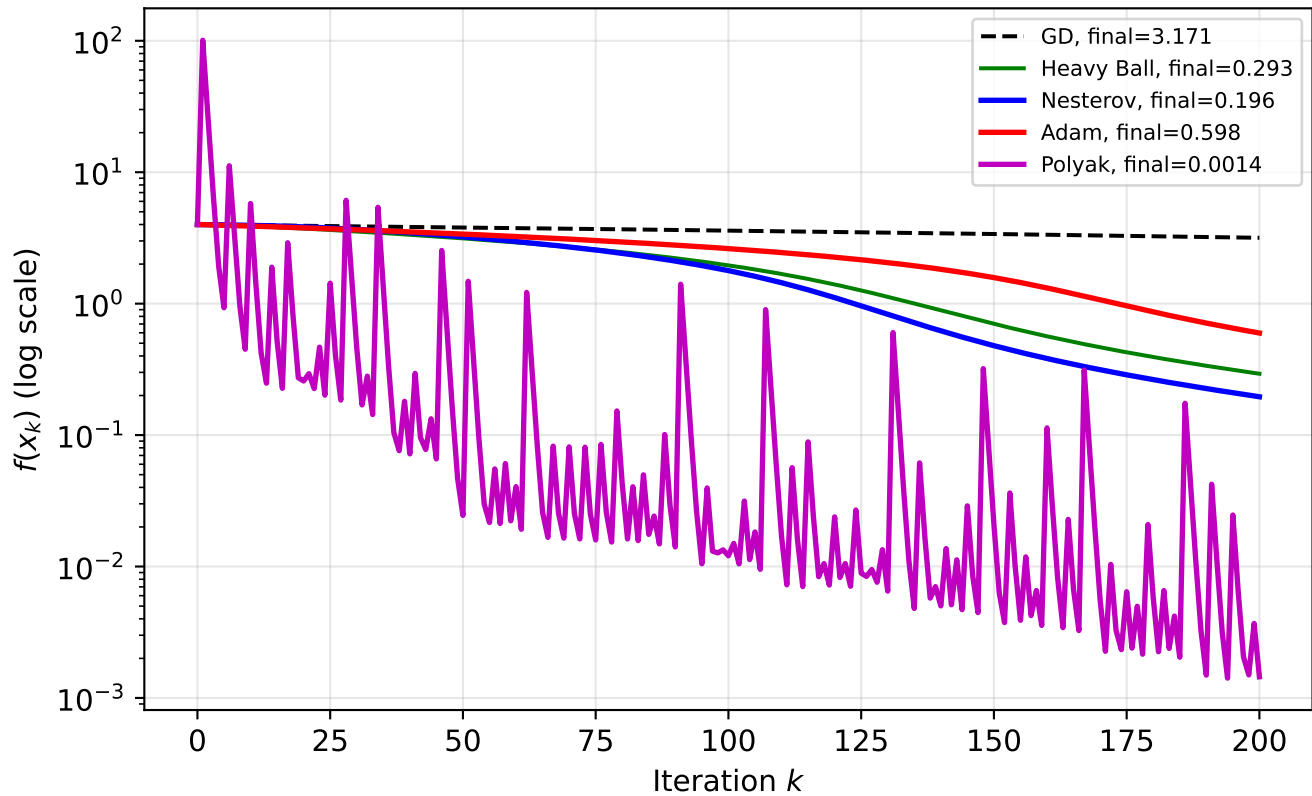
Benchmark C (Rosenbrock): All First-Order Methods, 200 iterations
