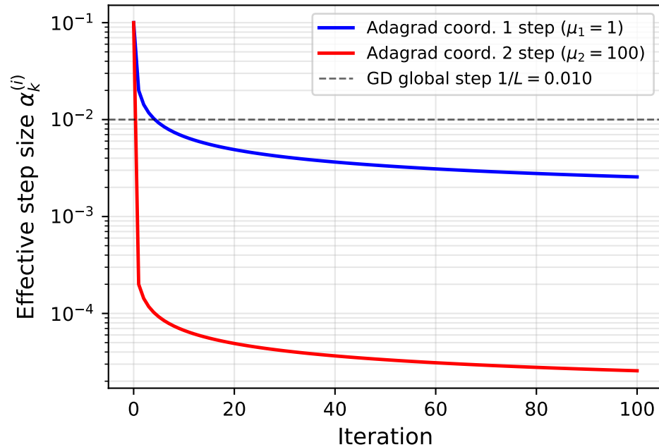
Per-coordinate Adagrad step sizes
