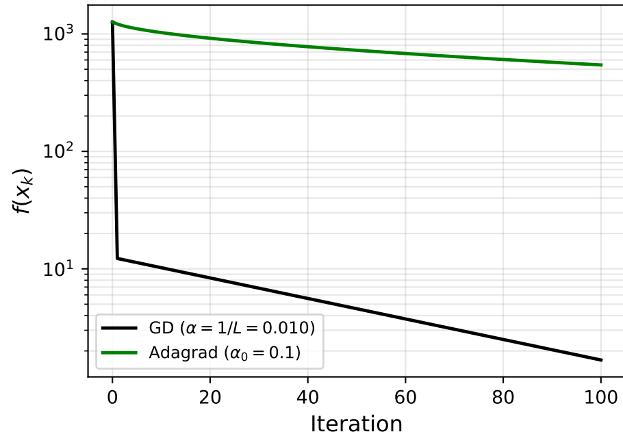
Convergence: Adagrad vs GD (anisotropic \mu_1 = 1, \mu_2 = 100 )
