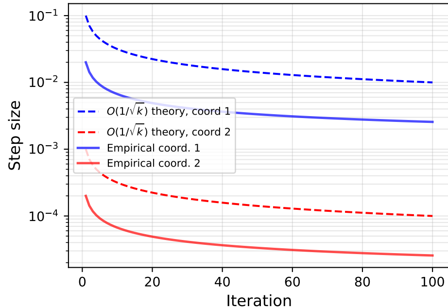
Theoretical O(1/\sqrt{k}) vs empirical decay
