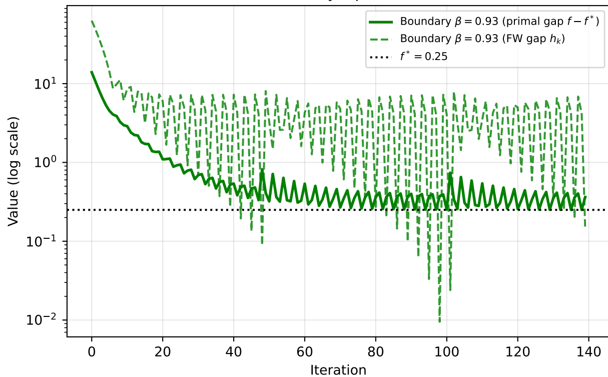
Q6-III: Primal Gap vs FW Duality Gap Boundary Optimum
