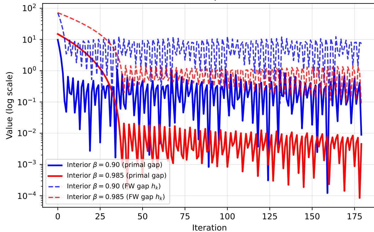
Q6-II: Primal Gap vs FW Duality Gap Interior Optimum
