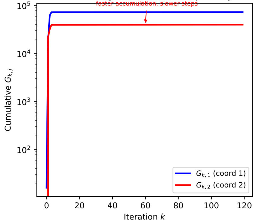
Adagrad Accumulator G_k (Monotone growth causes step decay)
