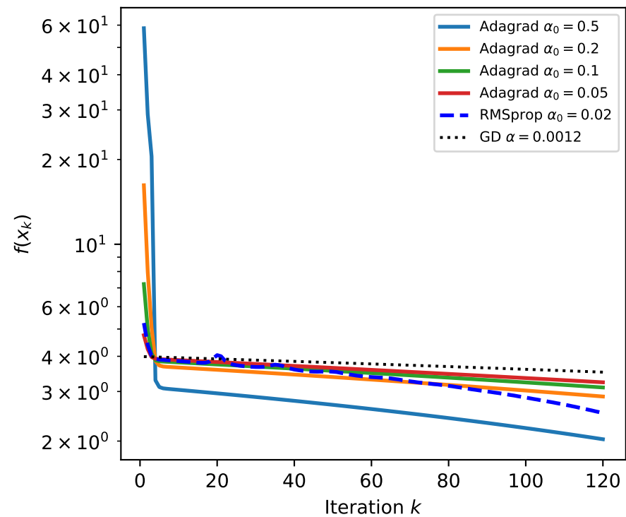
Adagrad: Sensitivity to \alpha_0 (Rosenbrock)
