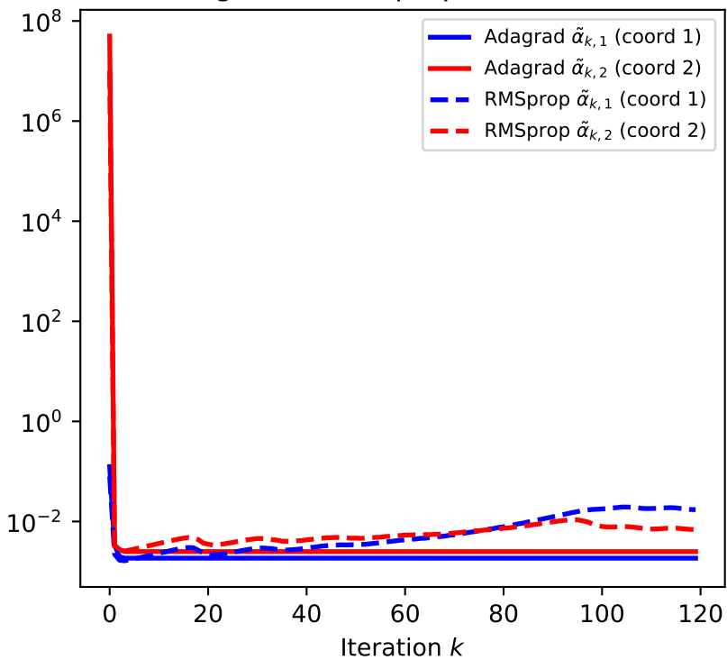
Per-Coordinate Step Sizes (Adagrad vs RMSprop, Rosenbrock)
