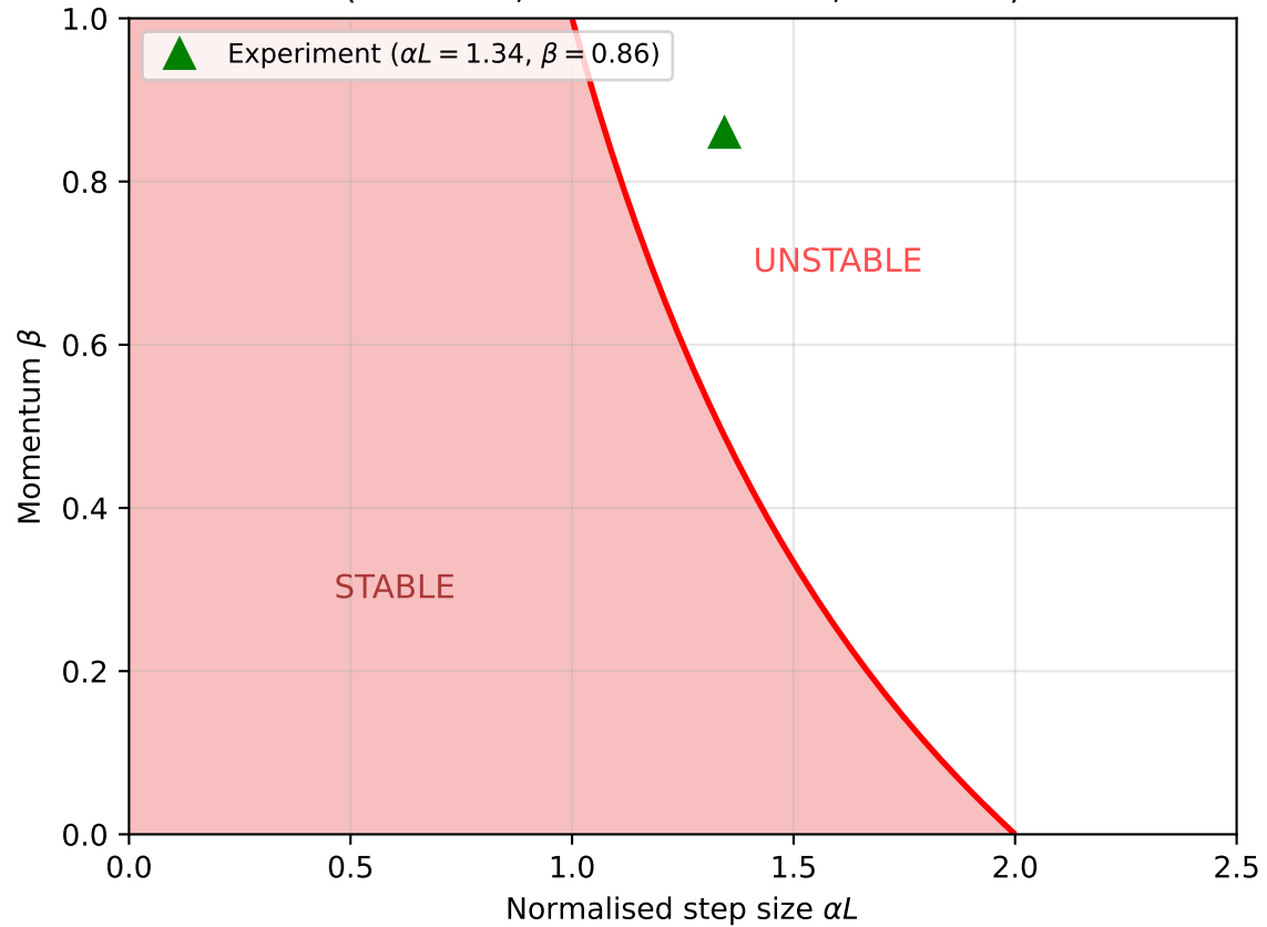
Heavy Ball Stability Region (Bench. C, L \approx 1680 at start, \kappa \approx 4200 )
