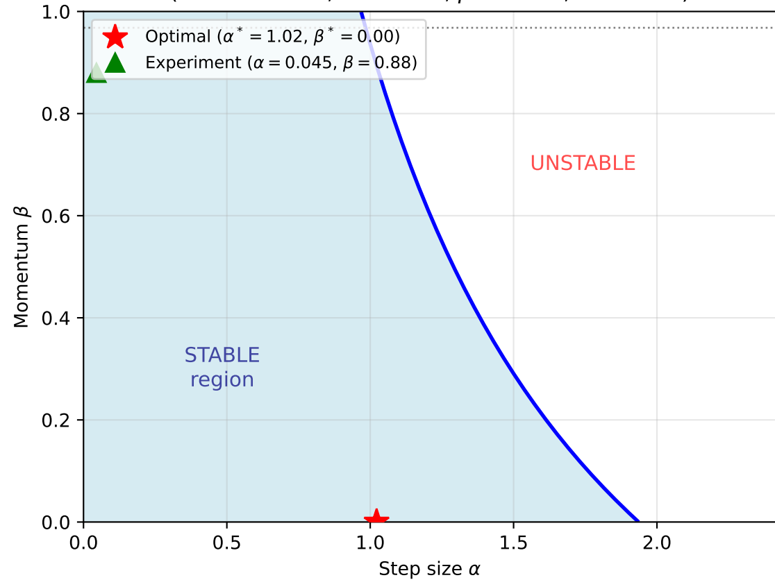
Heavy Ball Stability Region (Benchmark A, L = 1.033 , \mu = 0.925 , \kappa = 1.117 )
