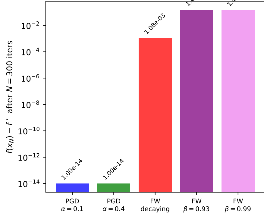
Final Suboptimality: FW vs PGD (300 iterations)
