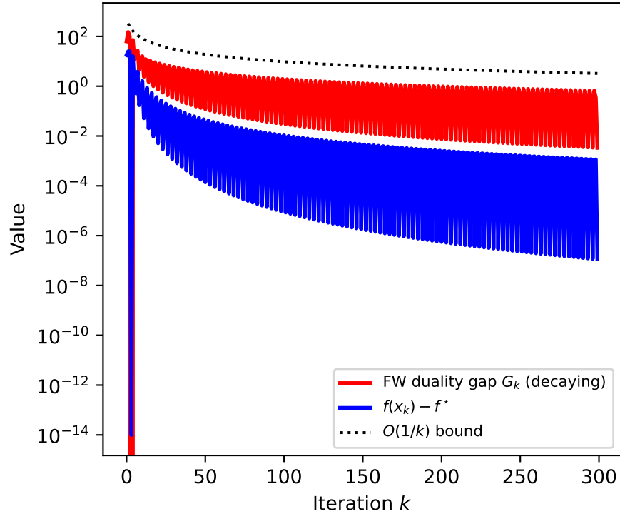
FW Duality Gap G_k = \nabla f^T(x_k - z_k) as Convergence Certificate
