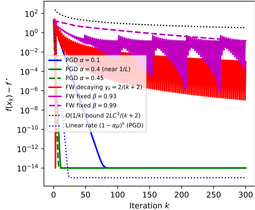
FW vs PGD: Boundary Optimum (f(x) = x_1^2 + x_2^2, x^* = (0.5, 0))
