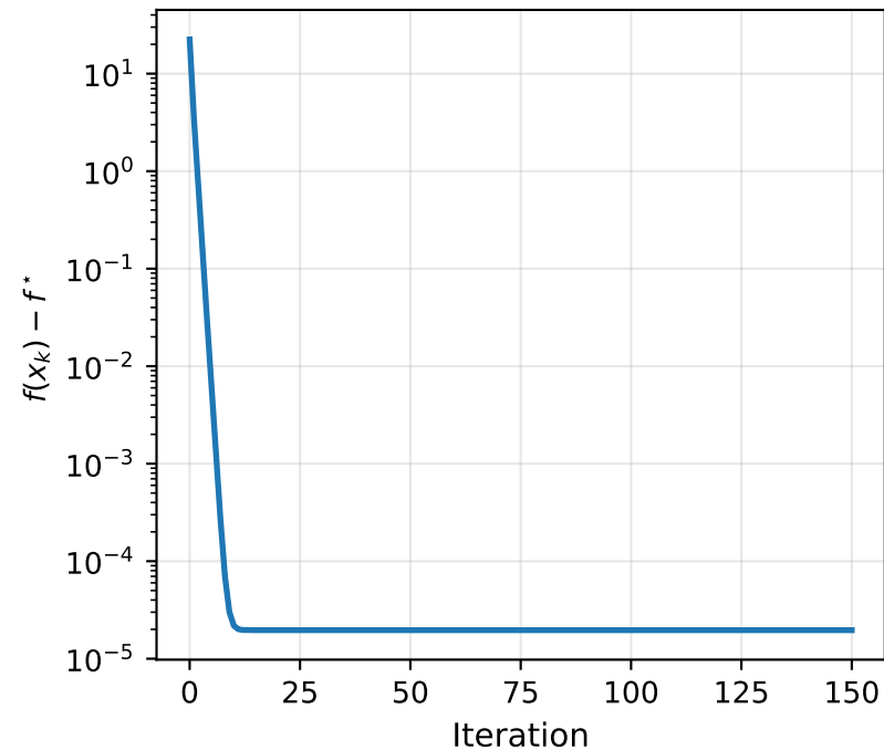
Adagrad convergence on Benchmark B
