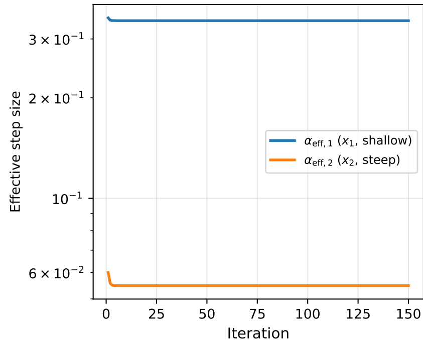
Per-coordinate effective learning rates
