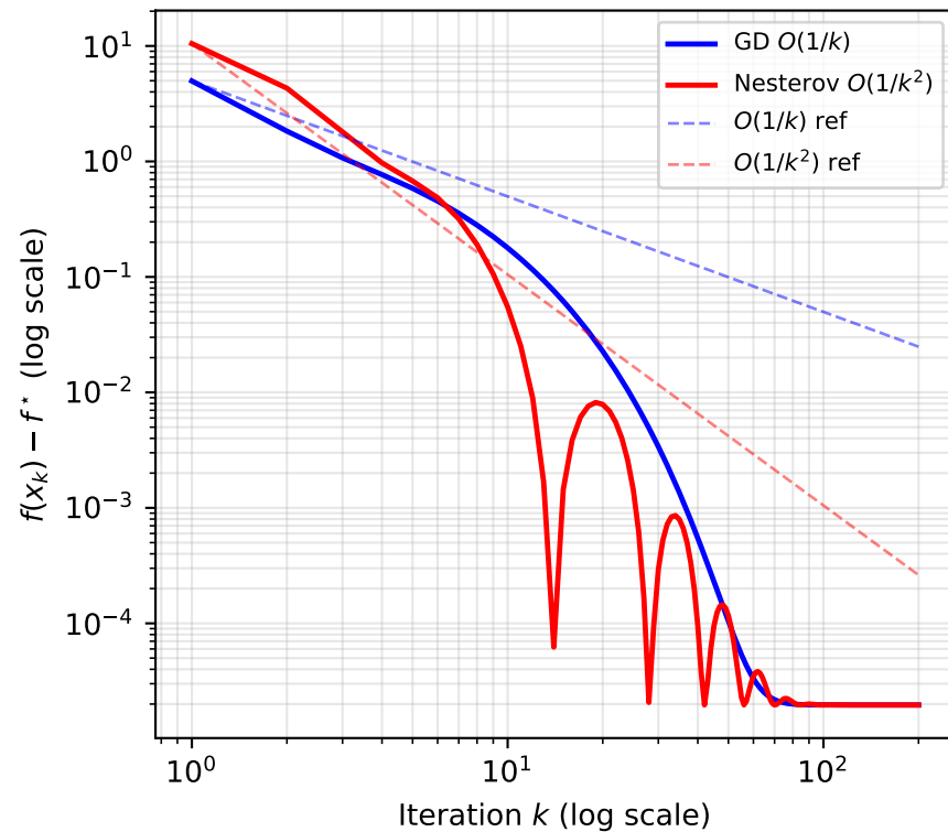
Benchmark B ( \kappa \approx 5 )
