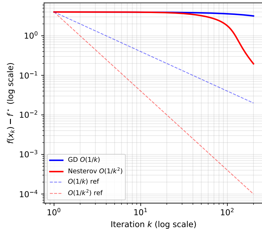
Benchmark C ( \kappa \approx 2004 )
