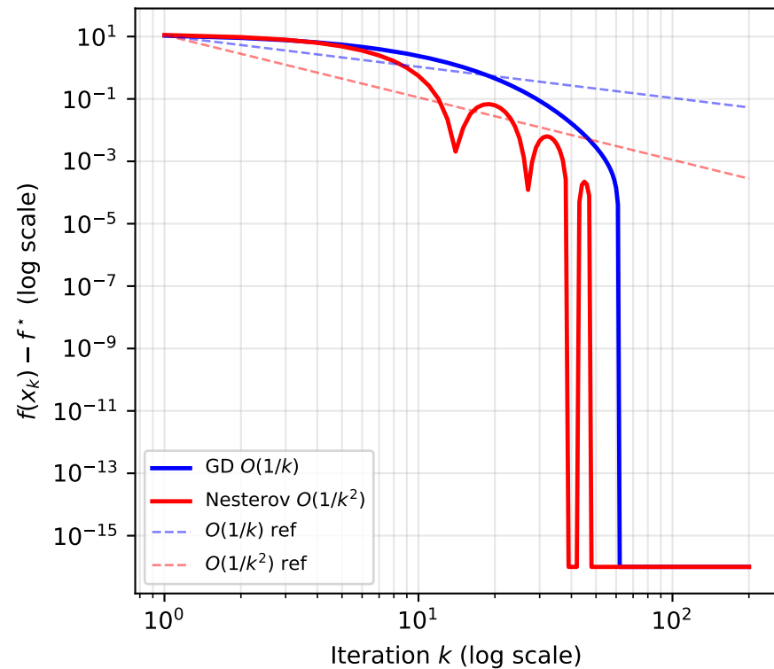
Benchmark A ( \kappa \approx 1 )
