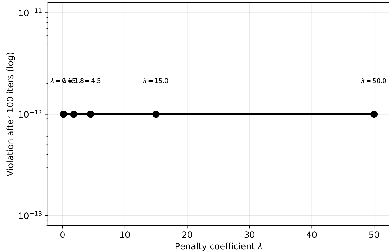
Final Violation vs \lambda (100 iterations)
