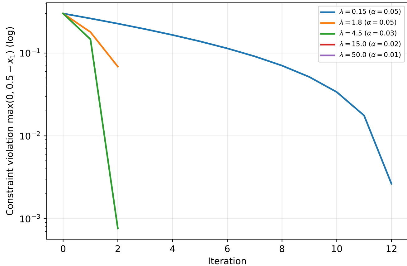
Penalty Method: Constraint Violation vs \lambda
