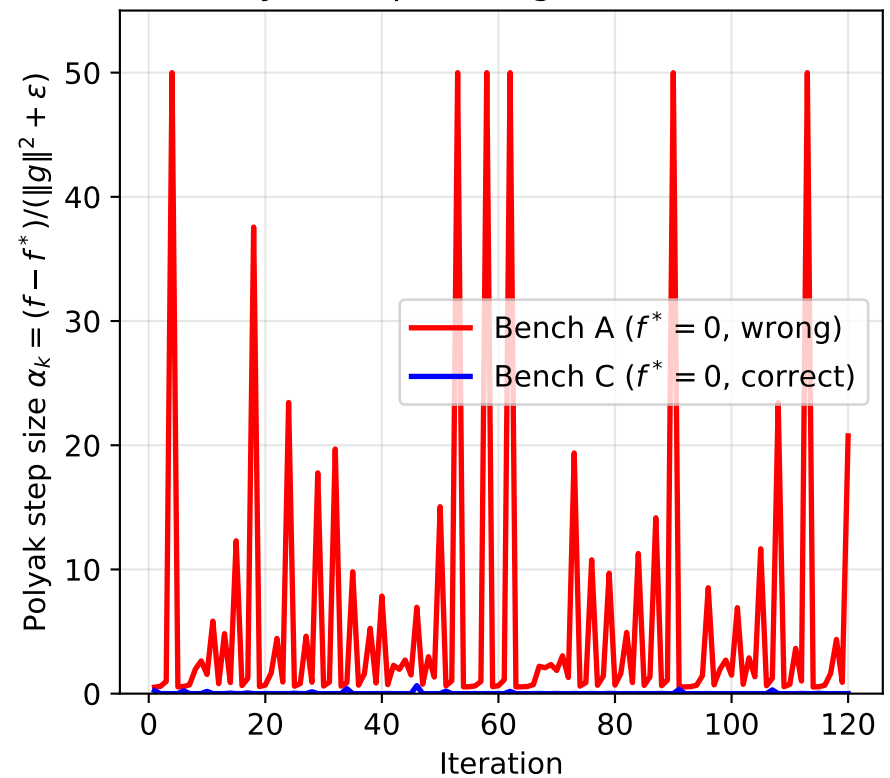
Polyak Step: Wrong vs Correct f^*
