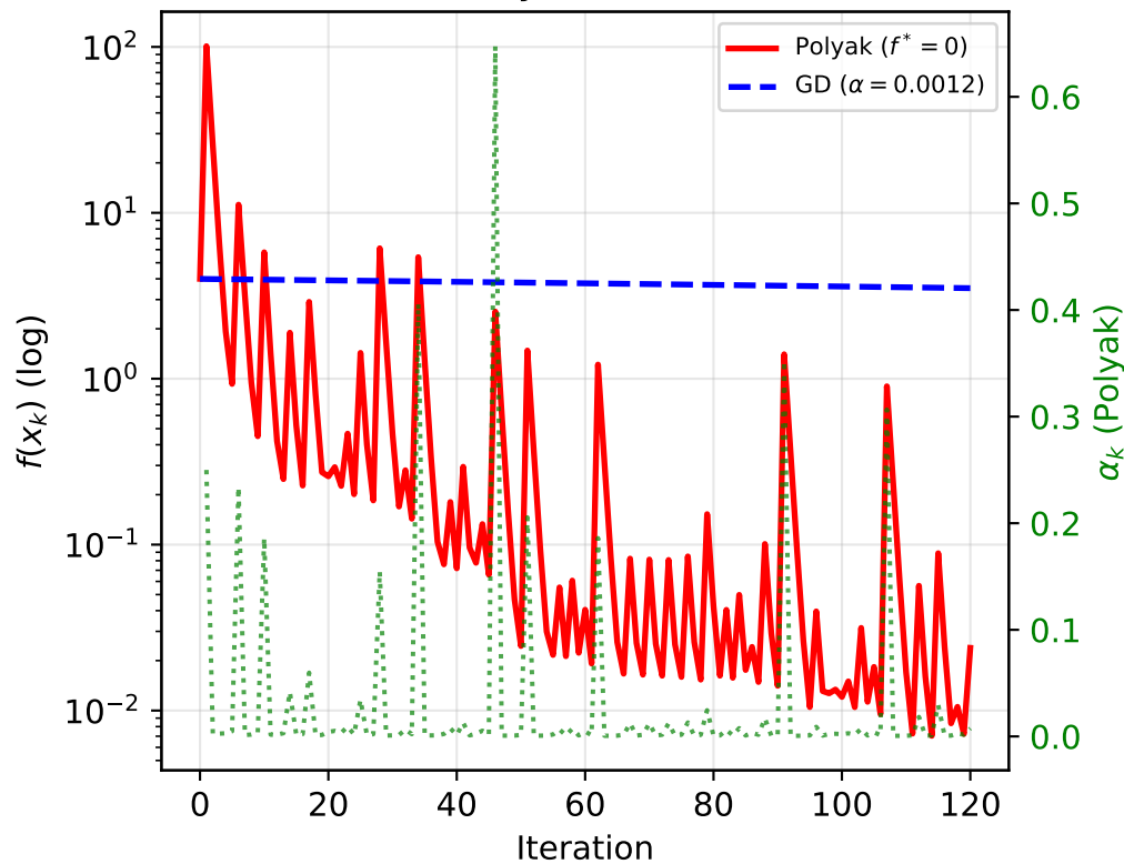
Bench C: Polyak (correct f^* = 0 )
