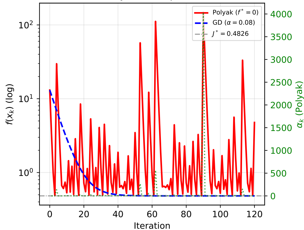
Bench A: Polyak (misspecified f^* = 0 )
