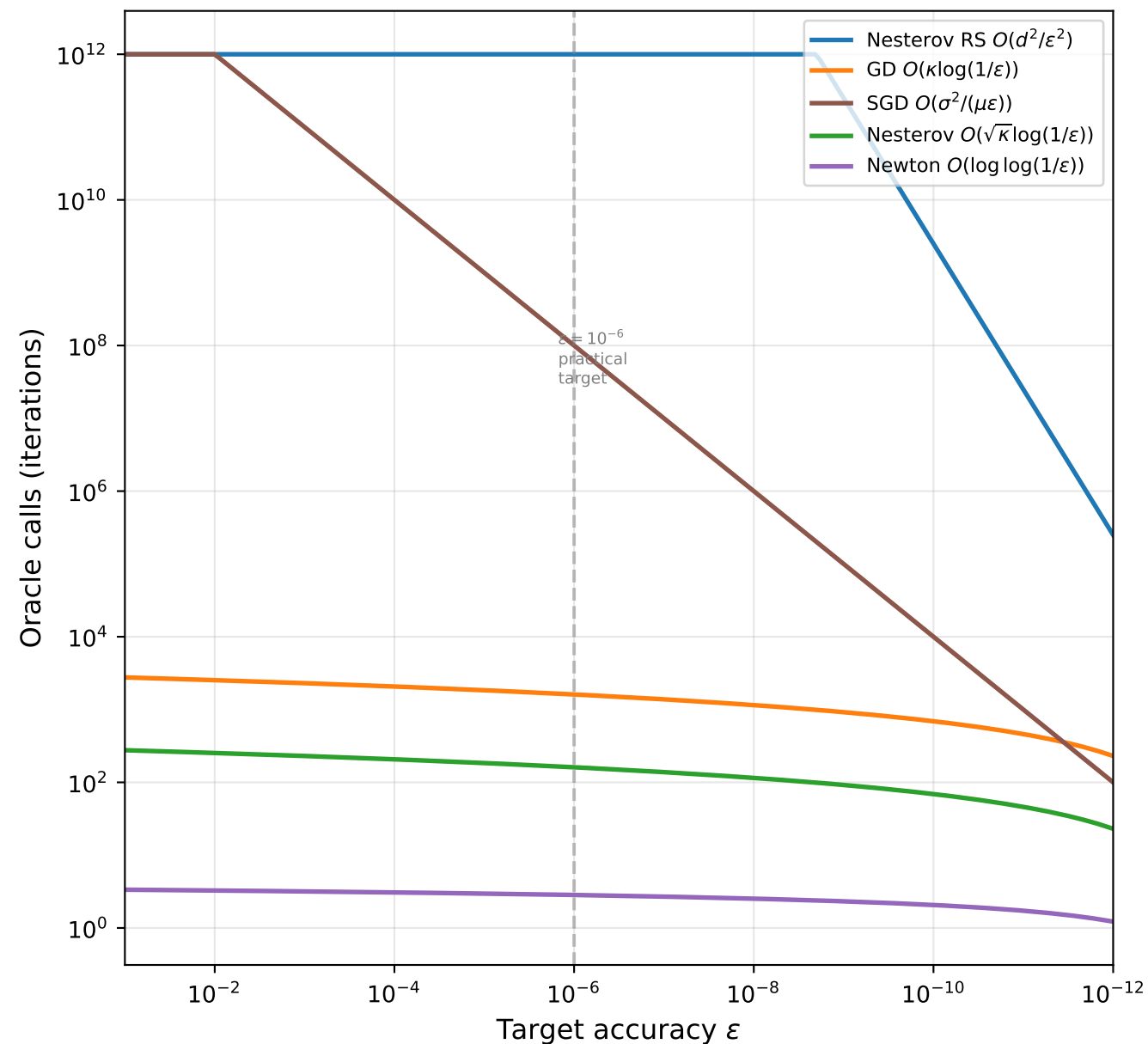
Oracle Complexity vs Target Accuracy ( \kappa = 100 , d = 50 )
