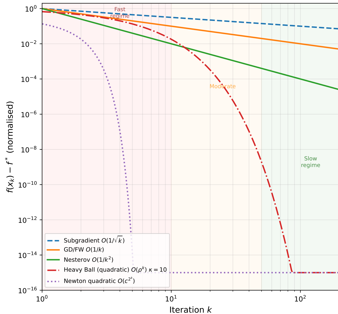
Convergence Rate Spectrum (All methods, normalised f(x_0) - f^* = 1 )
