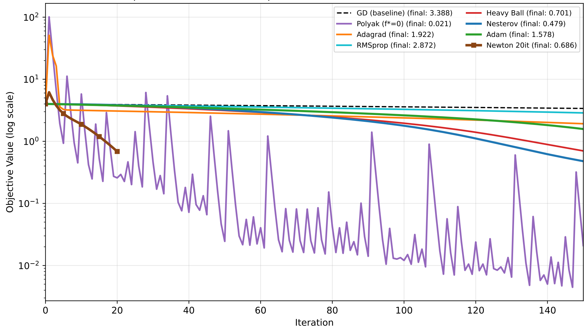
Comprehensive Method Comparison: Benchmark C (Rosenbrock, \kappa \approx 2500 )
