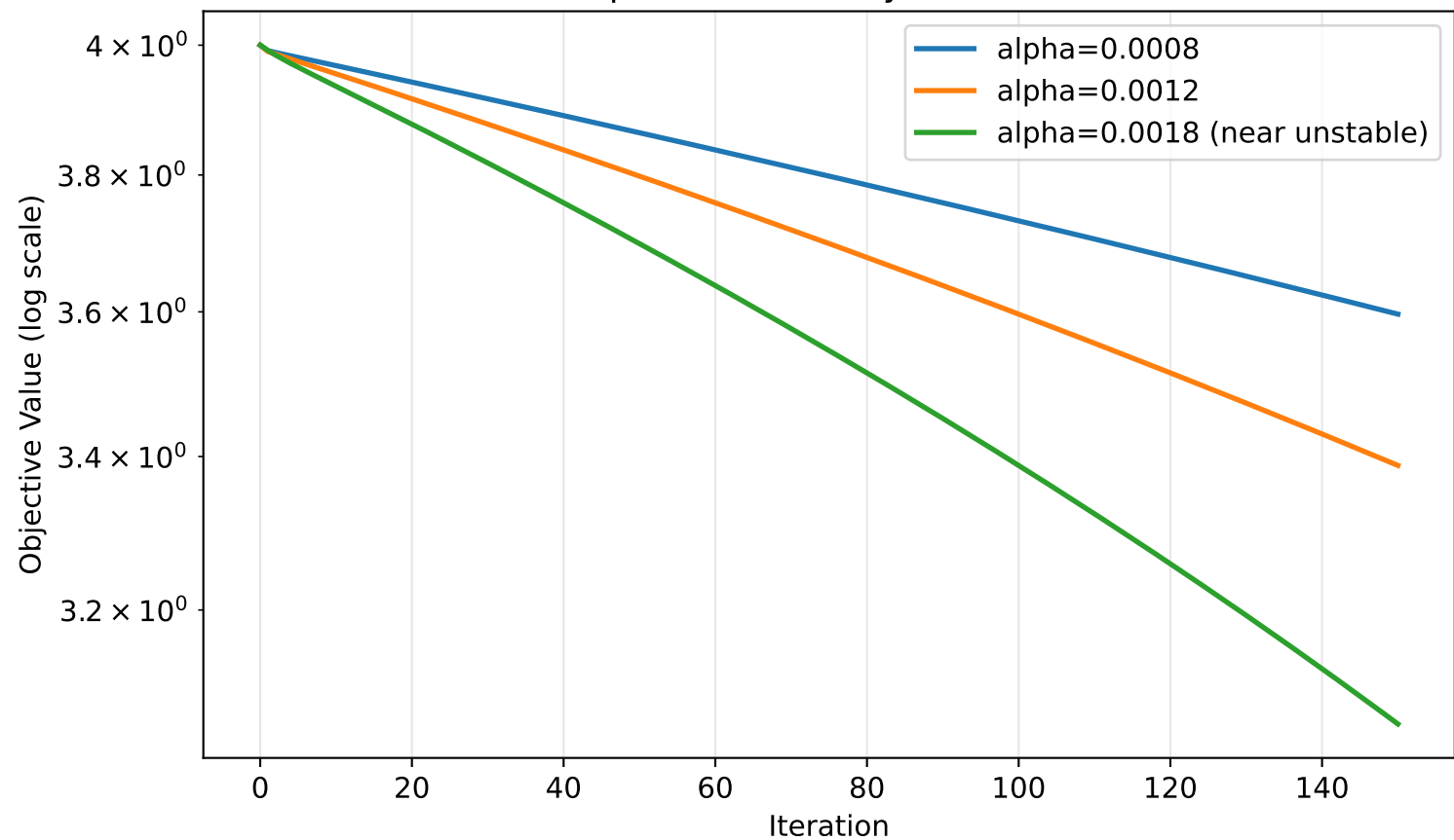
GD Step-Size Sensitivity on Rosenbrock
