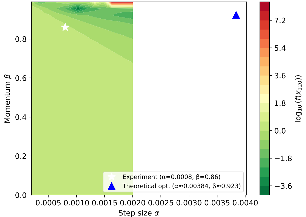
Heavy Ball stability map: f(x_{120}) on Rosenbrock
