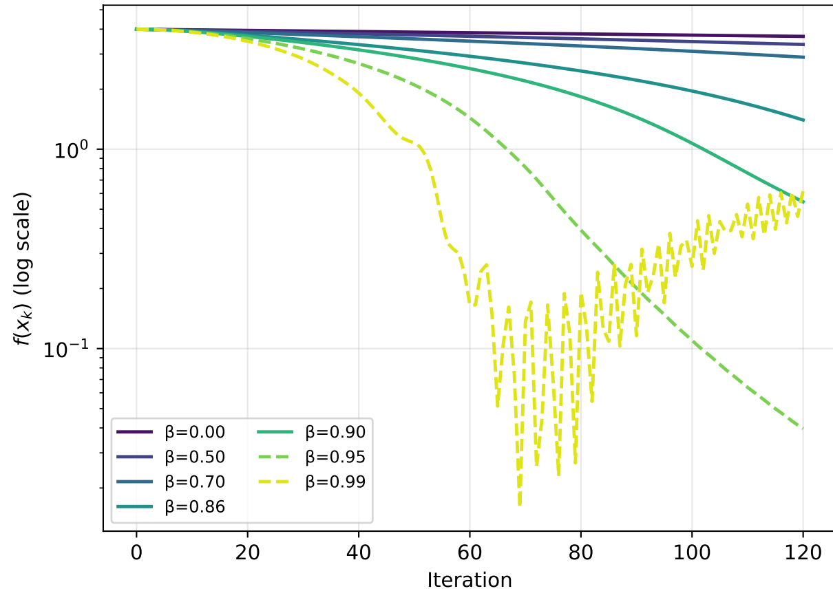
Heavy Ball: effect of momentum \beta on Rosenbrock ( \alpha = 0.0008 )
