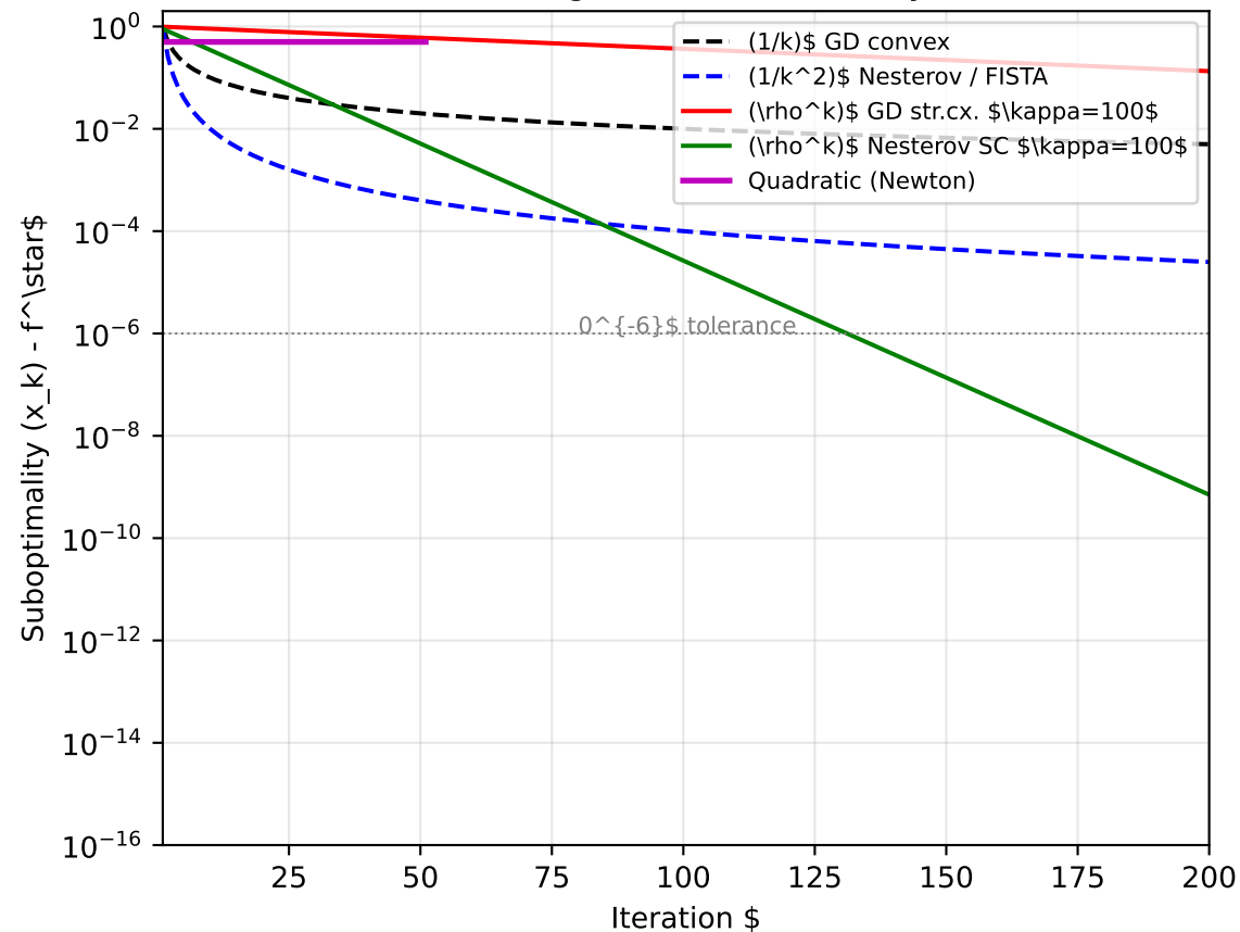
Convergence rate hierarchy
