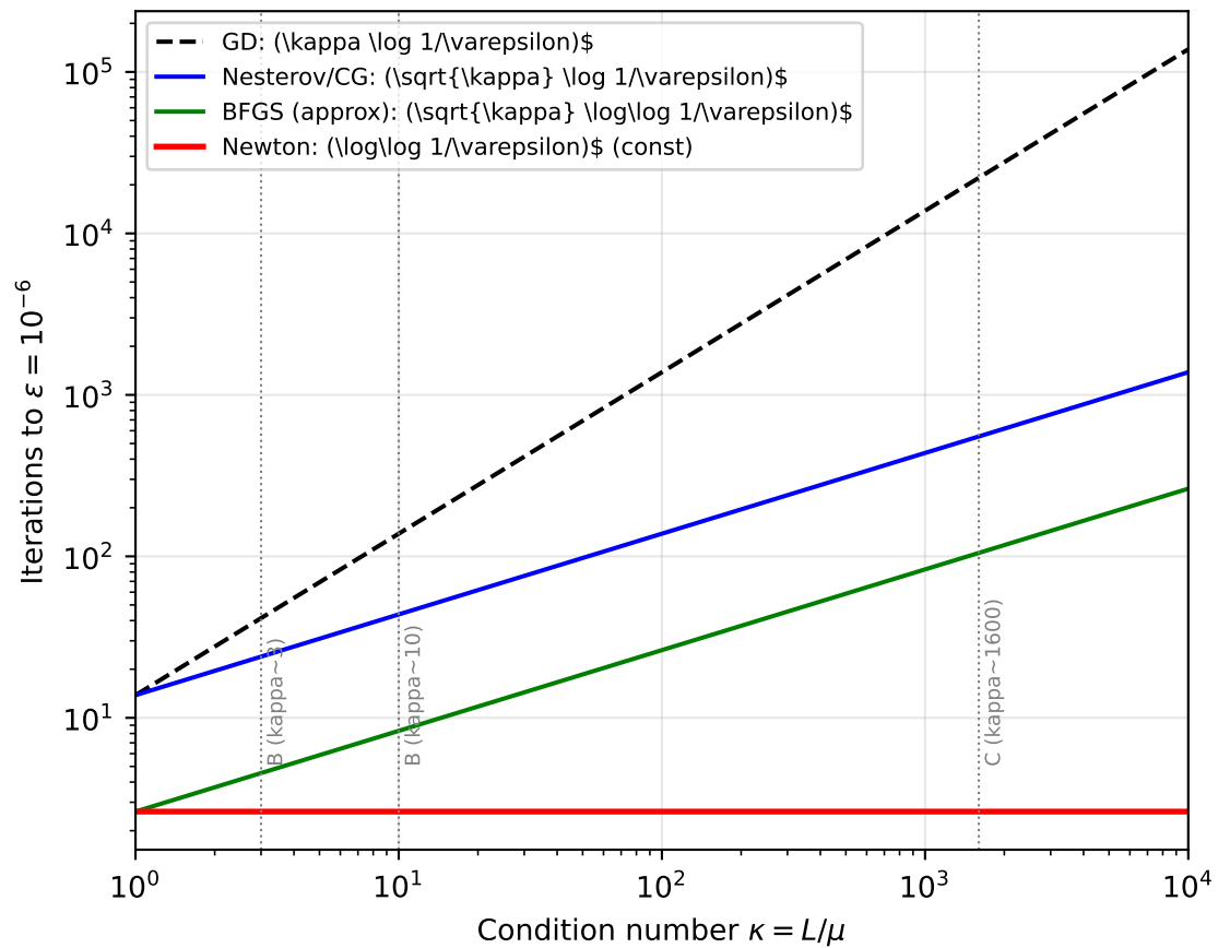
Oracle complexity vs condition number ( \varepsilon = 10^{-6} )
