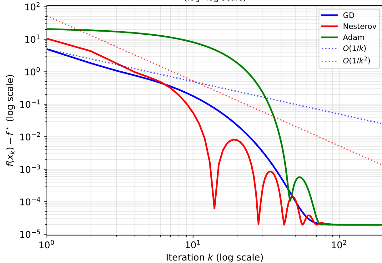
Q2: Convergence Rate Verification — Benchmark B (log-log scale)
