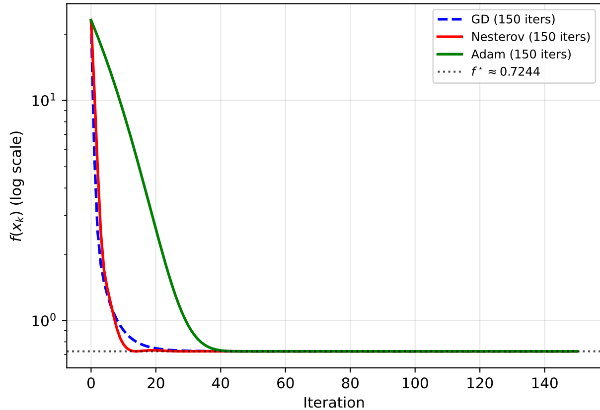
Q2: Convergence Comparison — Benchmark B (semi-log scale)
