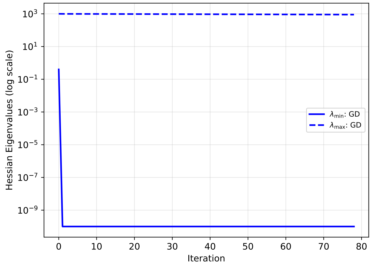
Q3: Rosenbrock Hessian Eigenvalues (GD Trajectory)
