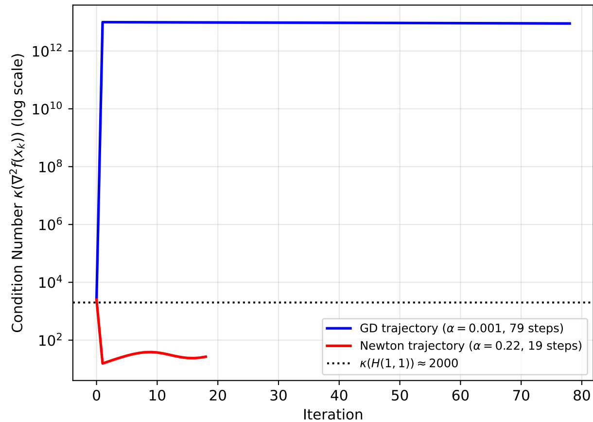
Q3: Rosenbrock Hessian Condition Number Along Trajectory
