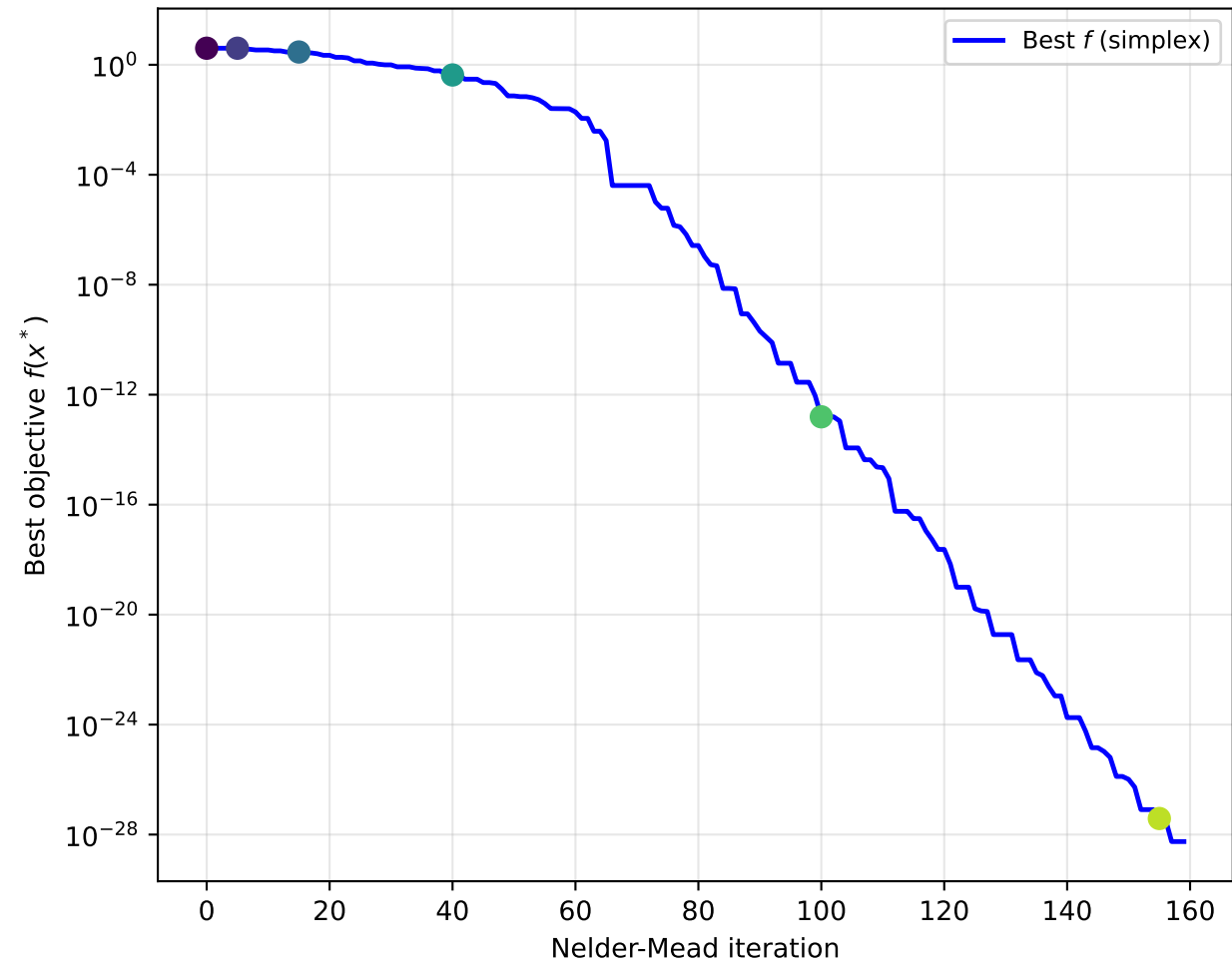
Nelder-Mead Convergence on Rosenbrock
