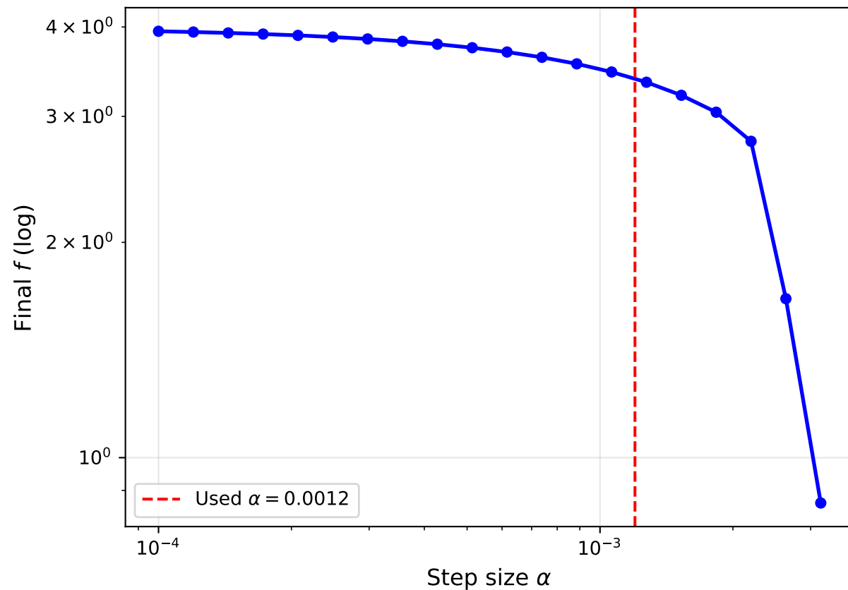
GD: sensitivity to \alpha
