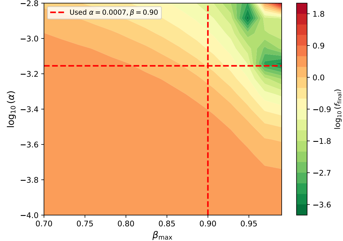
Nesterov: \alpha \times \beta_{\max} sensitivity
