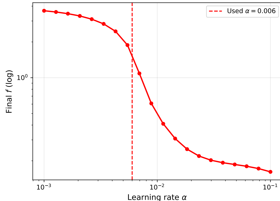
Adam: sensitivity to \alpha
