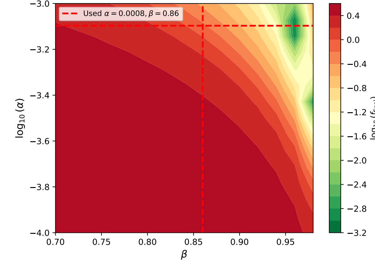
Heavy Ball: \alpha \times \beta sensitivity
