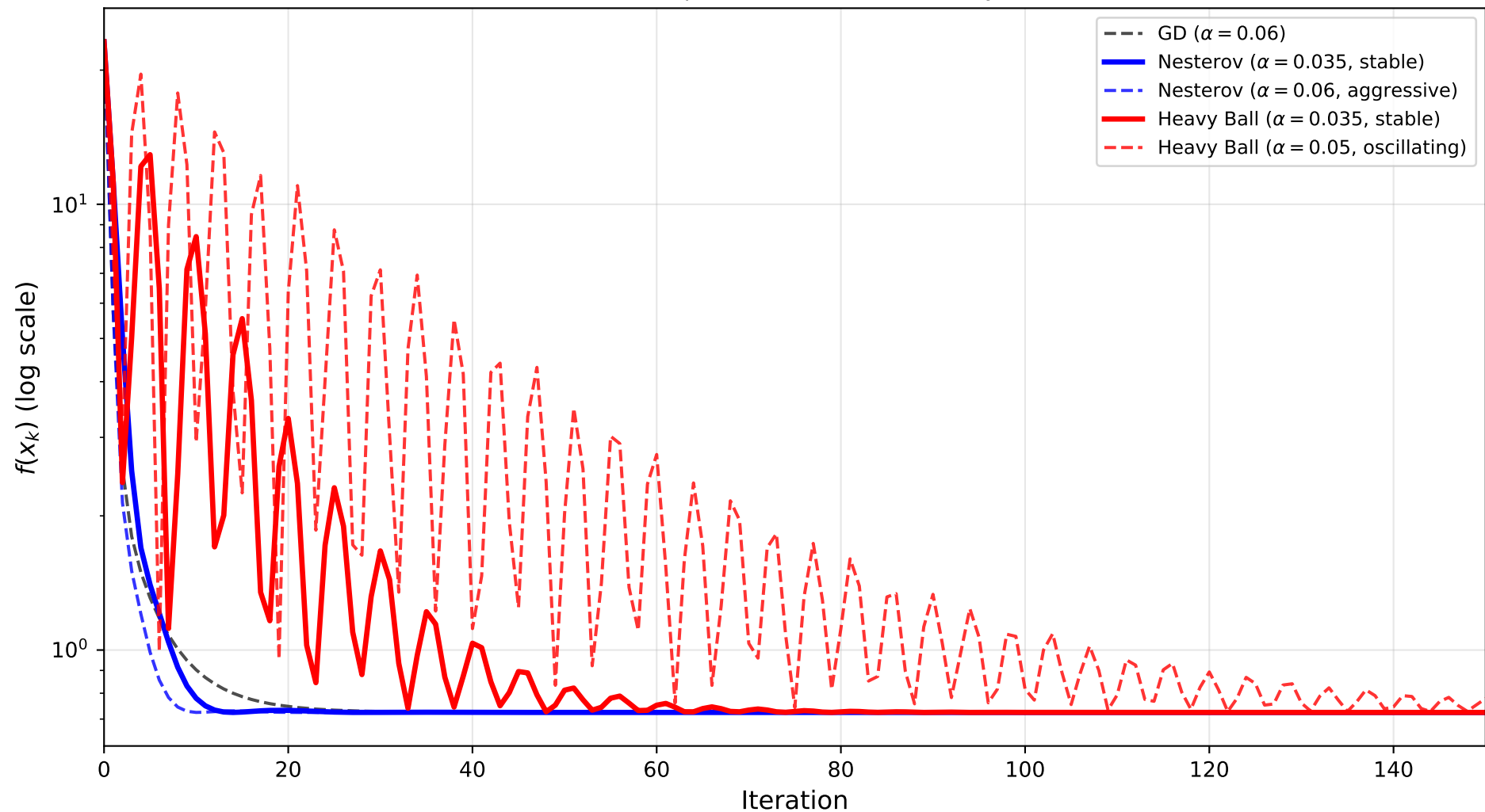
Q2: Nesterov vs Heavy Ball — Stability Comparison on Benchmark B Nesterov with lookahead prevents overshoot; Heavy Ball can oscillate
