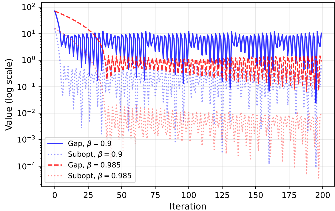
FW Gap g_k \geq f(x_k) - f^* (certified bound)
