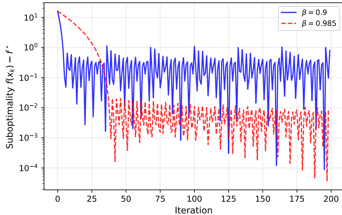
FW Suboptimality vs Iteration
