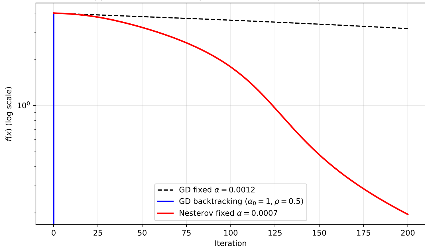
Q1 Supplement: Backtracking Line Search vs Fixed Step (Benchmark C)
