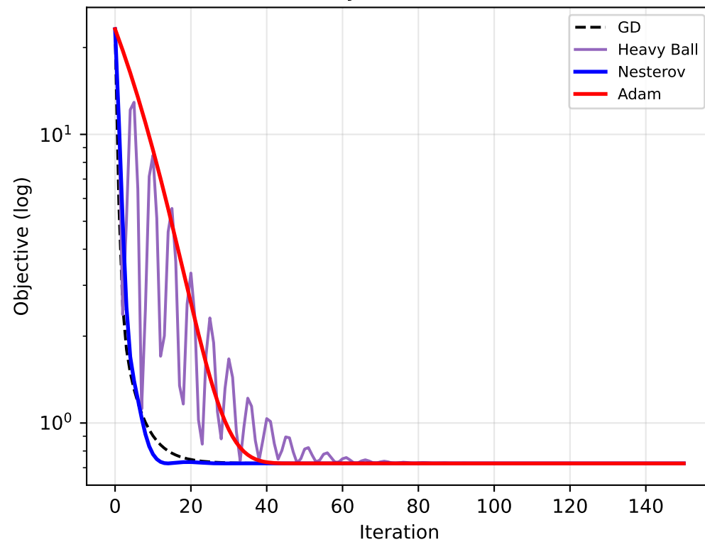
Benchmark B (Toy NN, \kappa \leq 10 )
