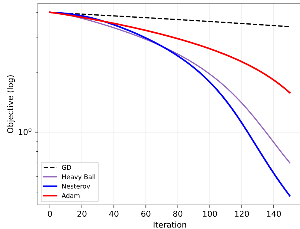
Benchmark C (Rosenbrock, \kappa \approx 2508 )
