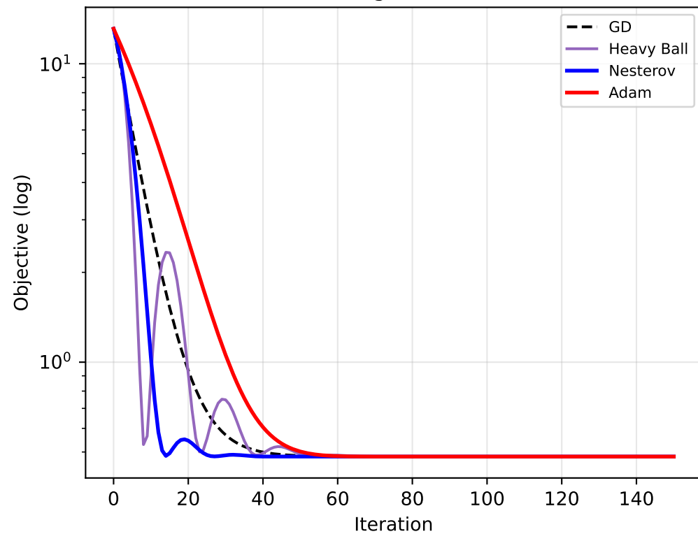
Benchmark A (Lin. Reg., \kappa \approx 1.12 )
