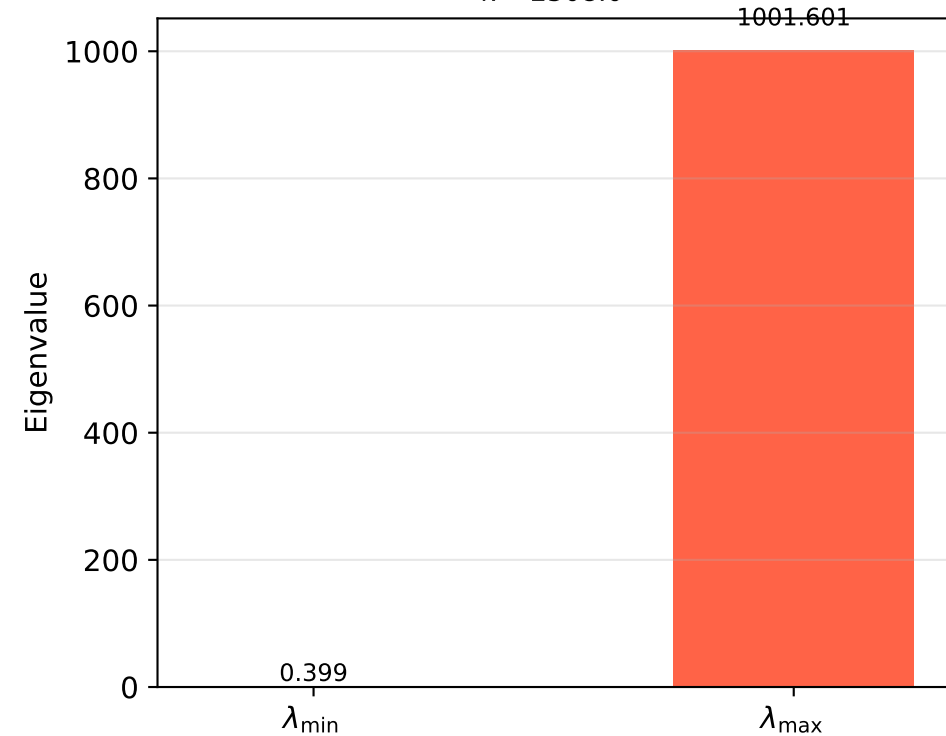
Bench. C: Rosenbrock at (1, 1) \kappa = 2508.0
