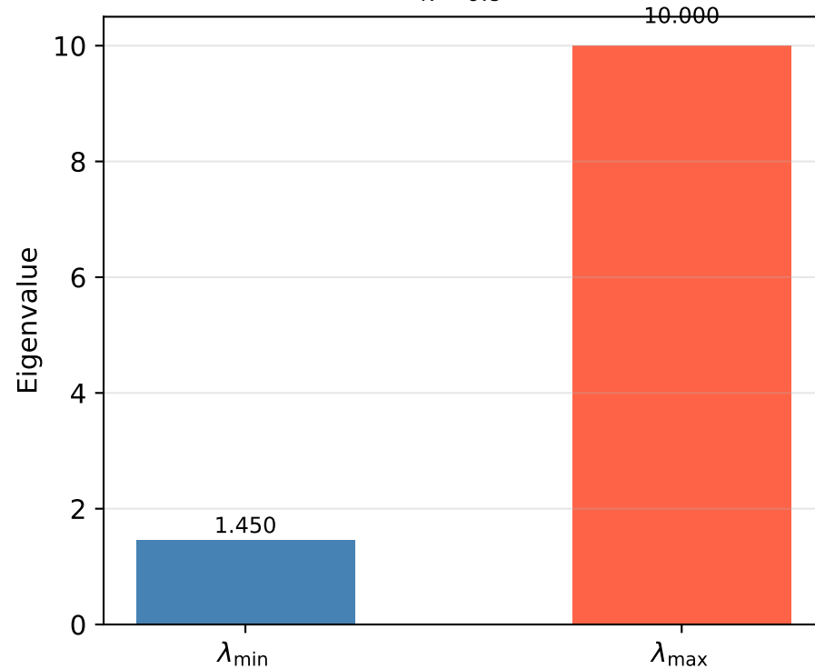
Bench. B: Toy Neural Network \kappa = 6.9
