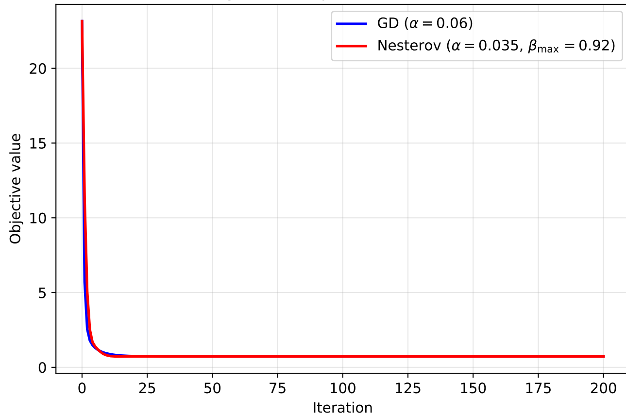
Convergence Comparison -- Benchmark B
