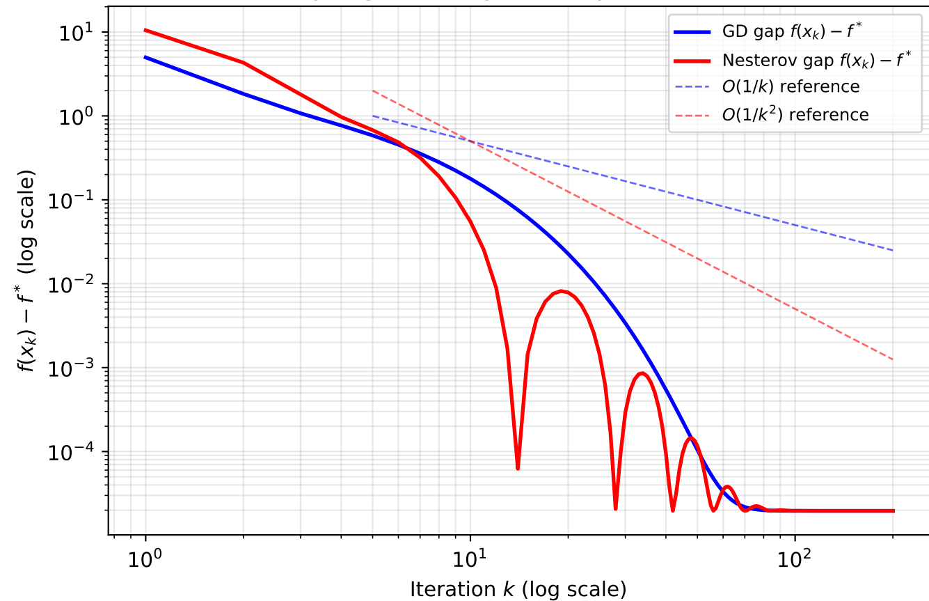
Log-Log: Convergence Gap vs Iteration
