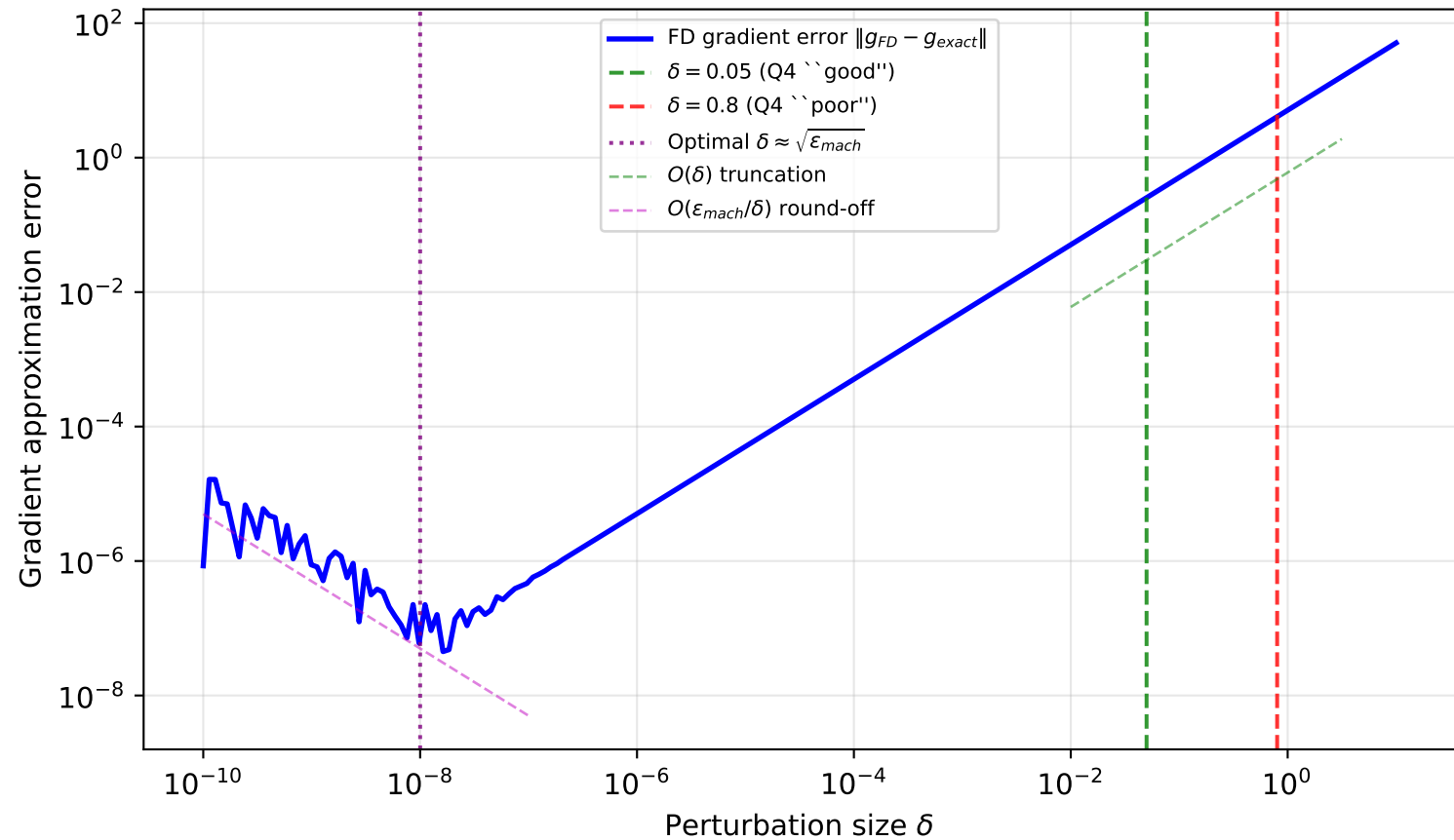
Q4: FD Gradient Error vs \delta at x = (0.5, 3.0)
