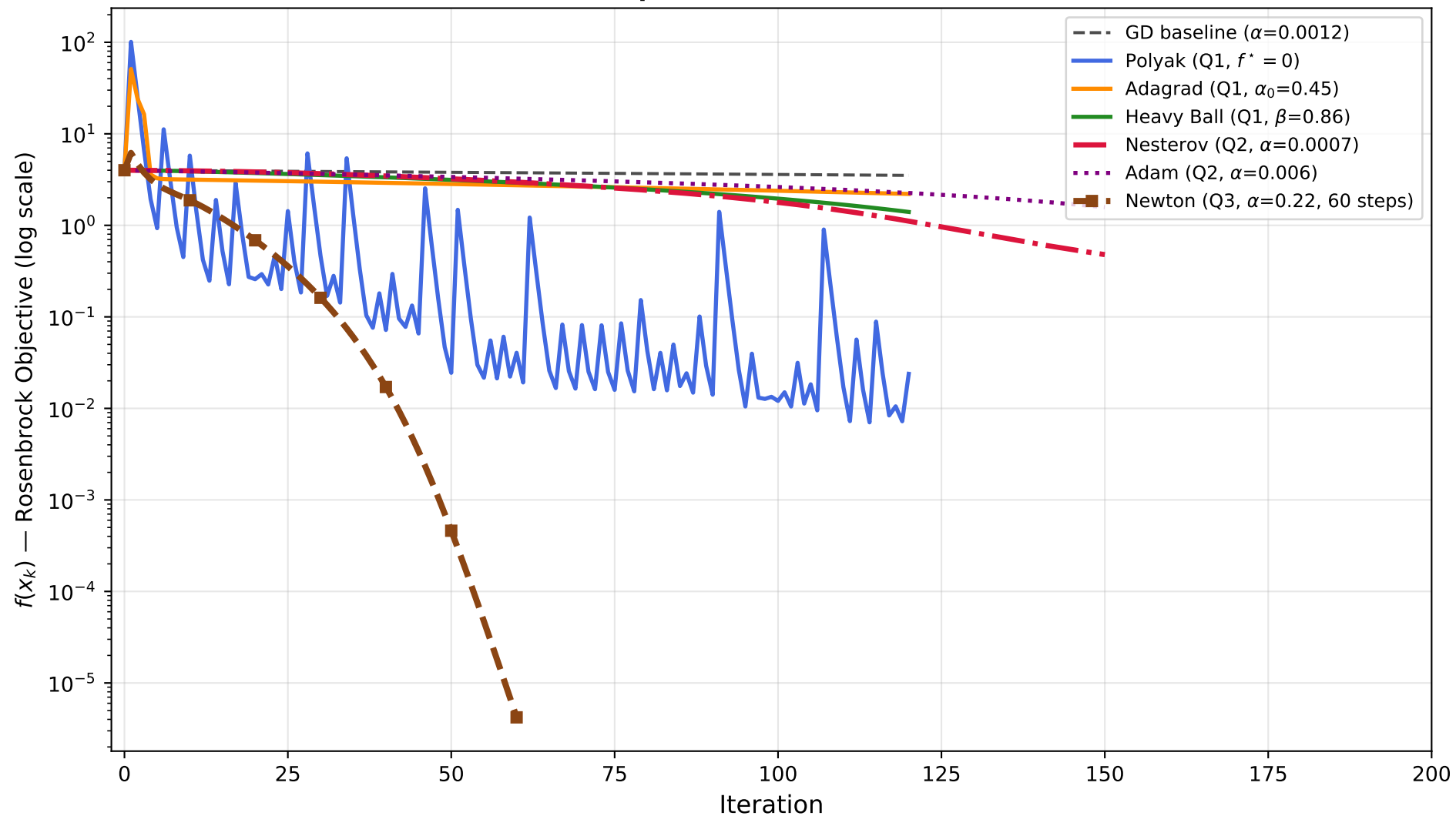
Cross-Question Method Comparison on Benchmark C (Rosenbrock Function)
