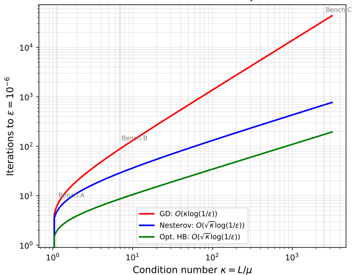
Iterations to Reach 10^{-6} Accuracy vs. \kappa
