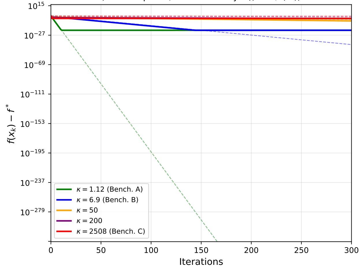
GD Convergence vs. Condition Number (solid: empirical, dashed: theory O((1 - 1/\kappa)^{2k}) )
