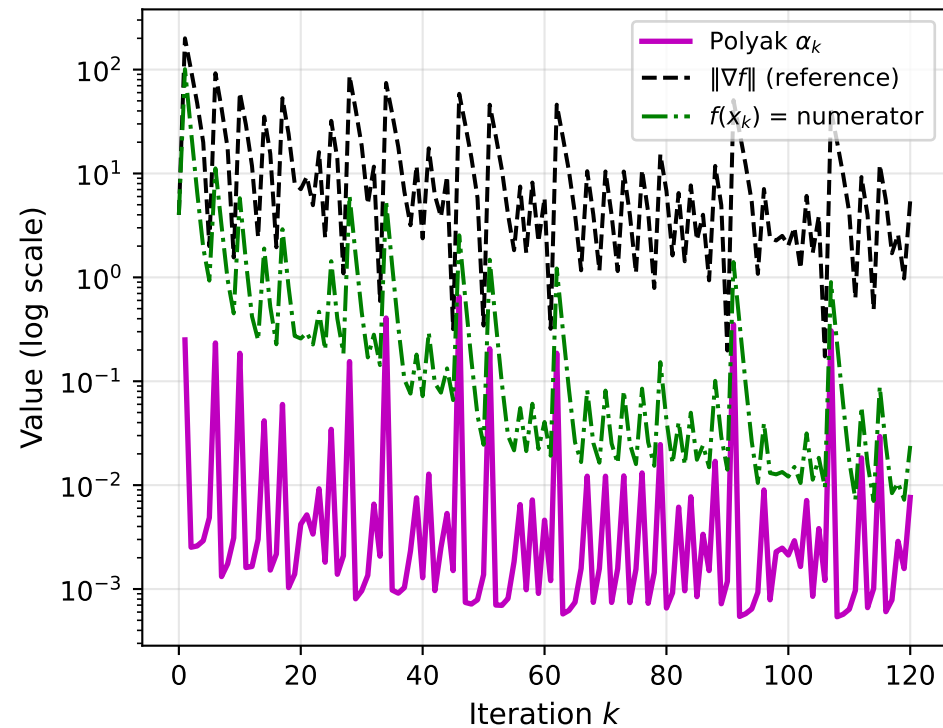
Polyak Step Dynamics (correct f^* = 0 ) \alpha_k = f(x_k)/(\|\nabla f\|^2 + \varepsilon)
