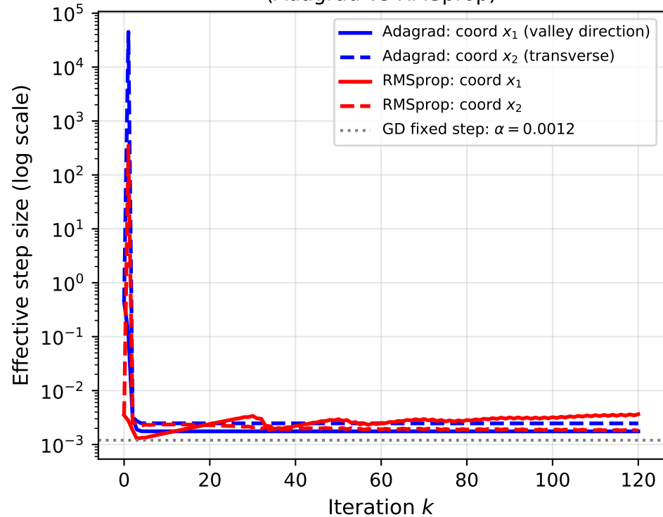
Per-Coordinate Effective Step Sizes (Adagrad vs RMSprop)
