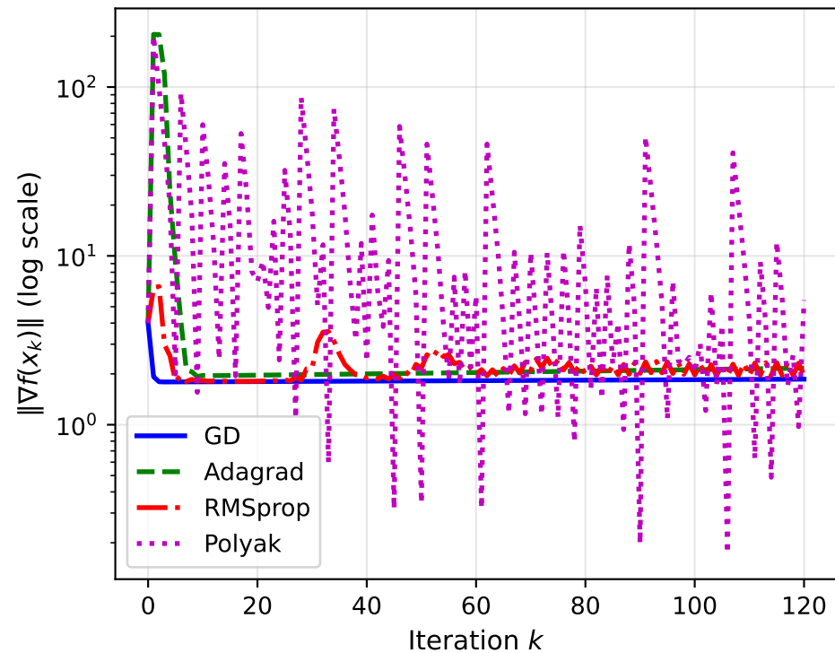
Gradient Norm Evolution (Benchmark C, Q = 120 iters)
