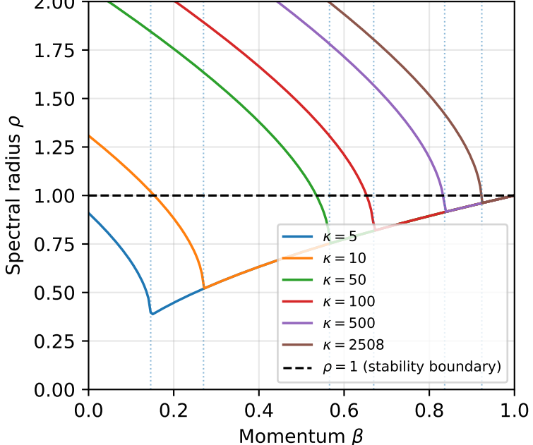
Heavy Ball Stability: \rho vs \beta
