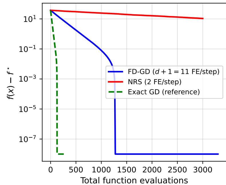
(b) d = 10 : NRS disadvantage grows ( \kappa = 1.4 )
