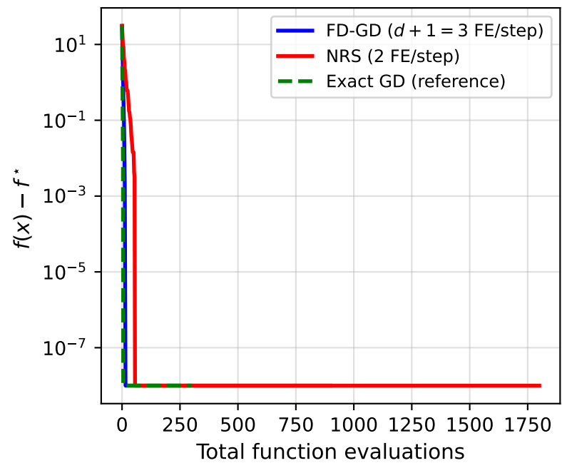
(a) d = 2 : NRS vs FD-GD ( \kappa = 0.9 )
