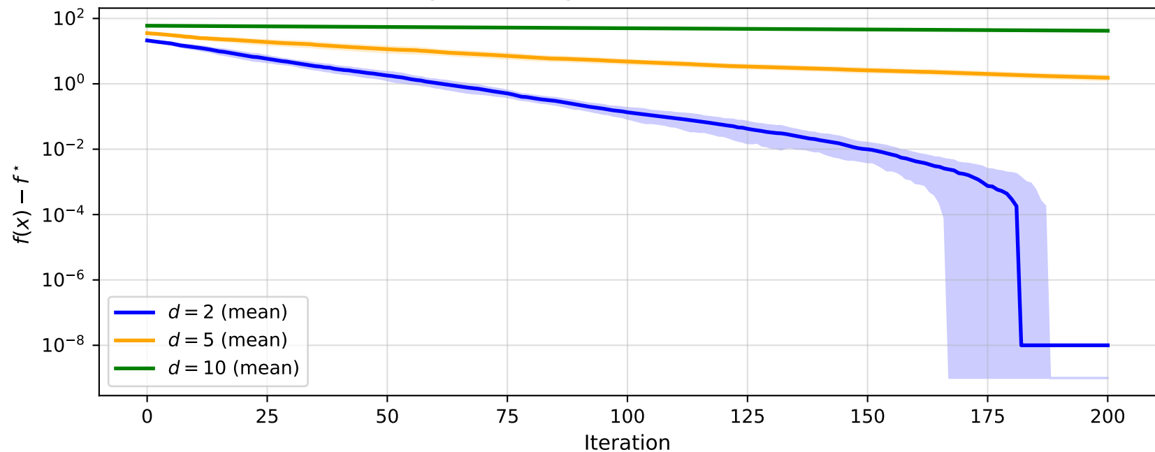
(d) NRS convergence vs dimension (mean \pm 1 std over 8 runs) Higher d \rightarrow larger variance, slower rate
