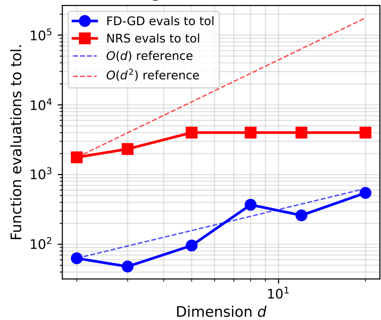
(e) Function evals to \varepsilon -accuracy ( \kappa = 10 , \varepsilon = 10^{-3} , factor of \log(1/\varepsilon) omitted)
