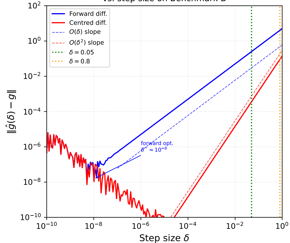
Gradient approximation error vs. step size on Benchmark B
