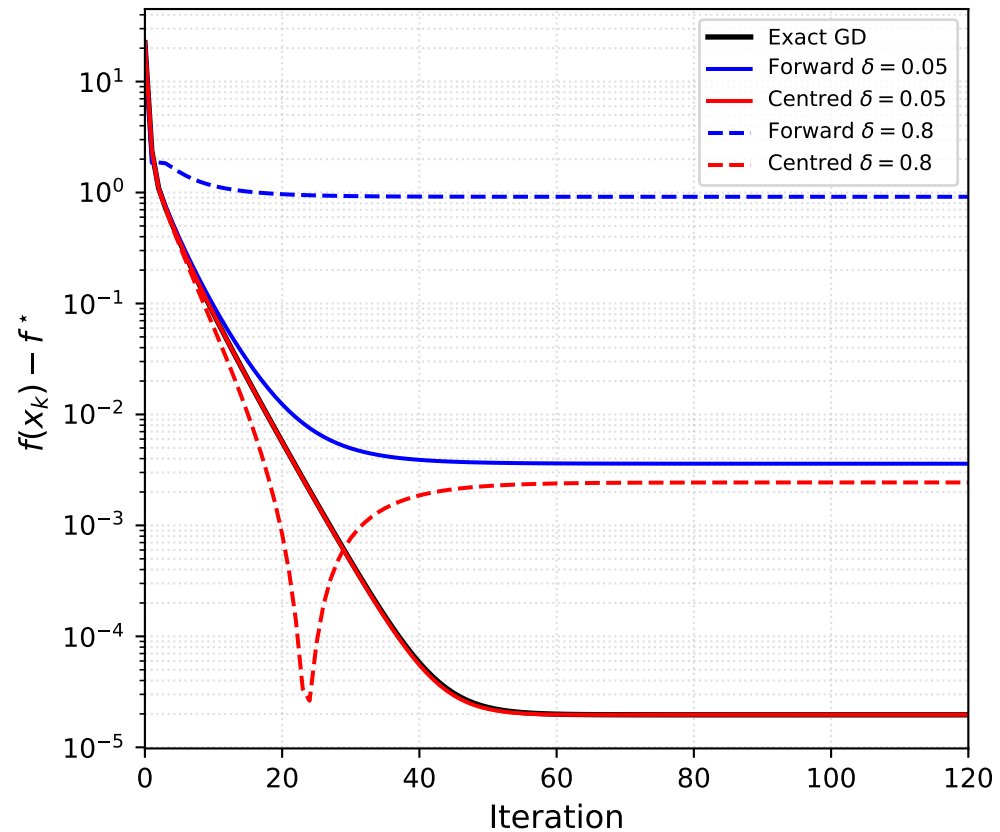
FD GD convergence: f(x_k) - f^* on Benchmark B
