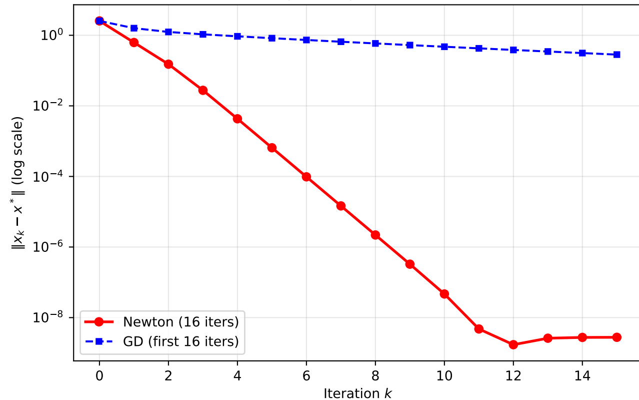
Q3: Convergence Speed — Benchmark B
