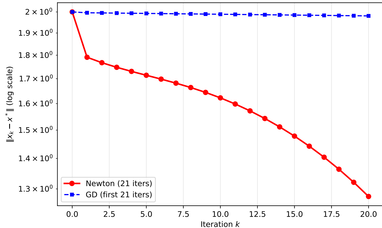
Q3: Convergence Speed — Benchmark C (Rosenbrock)
