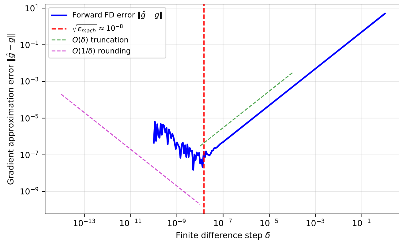
Q4: FD Gradient Error vs \delta (Benchmark B, x = (0.5, 2.5) )
