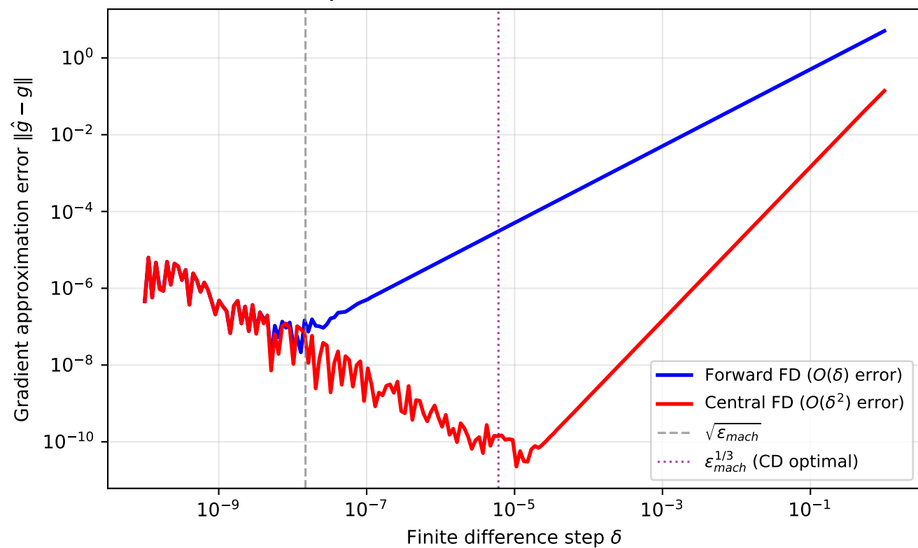
Q4: Forward vs Central Differences
