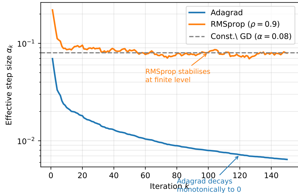
Effective Step Size: Adagrad vs RMSprop
