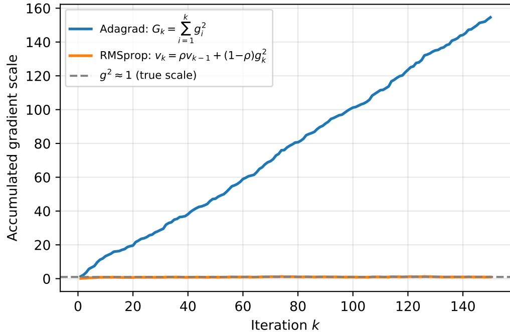
Gradient Accumulation: Cumulative vs EMA
